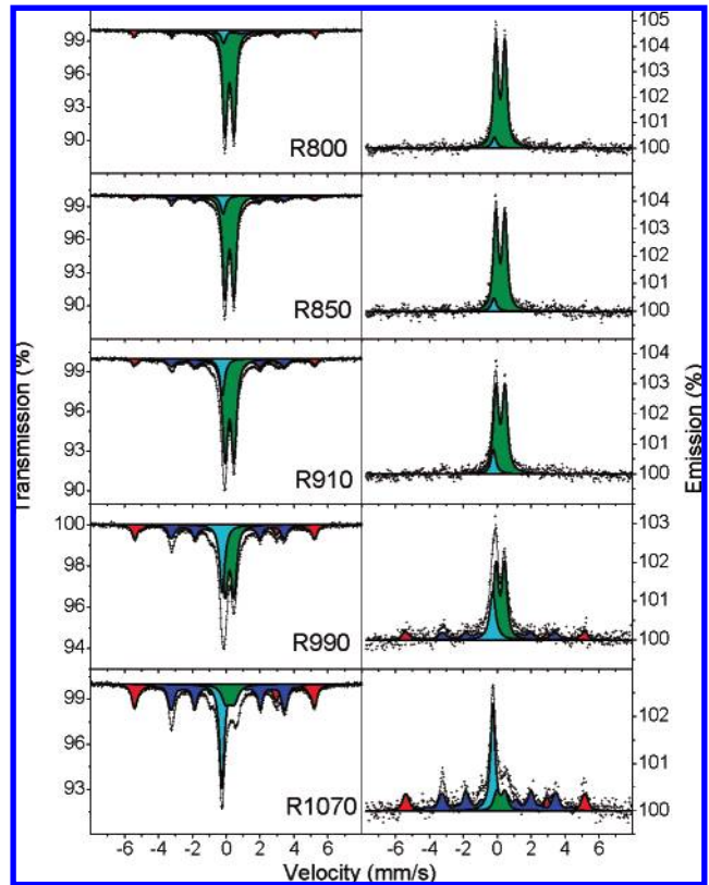
Figure 1. Transmission (left) and emission (right) spectra of the nanocomposites powders measured at room temperature. \alpha -Fe (red); \text{Fe}_3\text{C} (blue); (\text{Al,Fe})_2\text{O}_3 (olive); \gamma -Fe-C (cyan).
