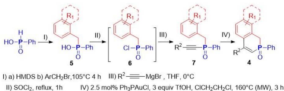
Scheme 1 Synthetic pathway of Isophosphinoline 2-oxides 4
