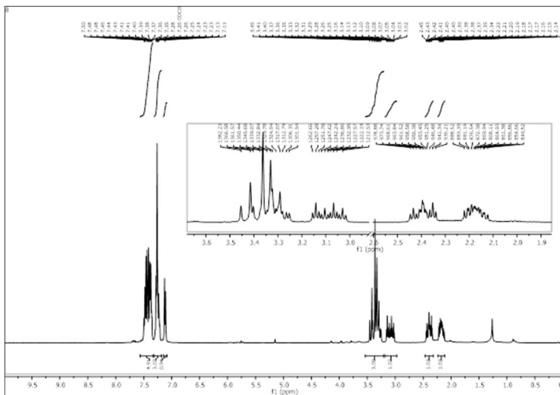
Figure 3 ^1\text{H} NMR spectra of compound 8
