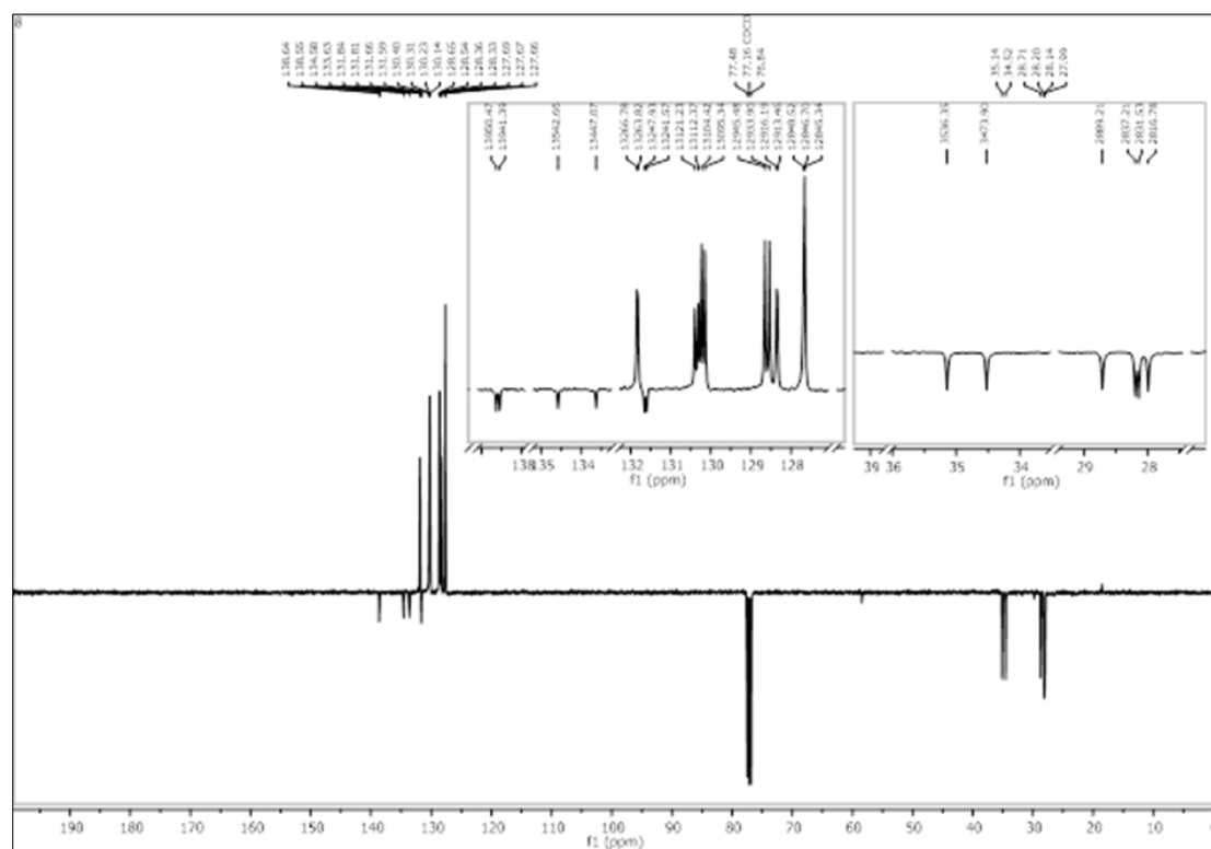
Figure 4 ^{13}\text{C} NMR spectra of compound 8
