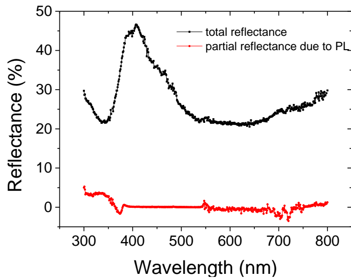
Figure 6: Total reflectance and partial reflectance due to the PL of a c-Si solar cell coated with [Eu(tta) 3 phen] in EVA.
