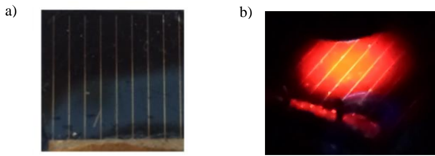
Figure 2: c-Si cell fabricated and coated with EVA including [Eu(tta) 3 phen] a) top-view b) illuminated at a wavelength of 350 nm.
