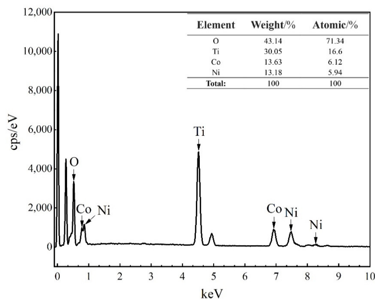
Figure 5. EDS spectrum of products calcined at 800 °C with a Co/Ni ratio of 0.5:0.5 (the analyzed area corresponds to the red box marked in Figure 4(c2)).
