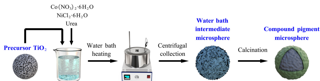
Figure 1. Process diagram for the preparation of composite pigment powders.
