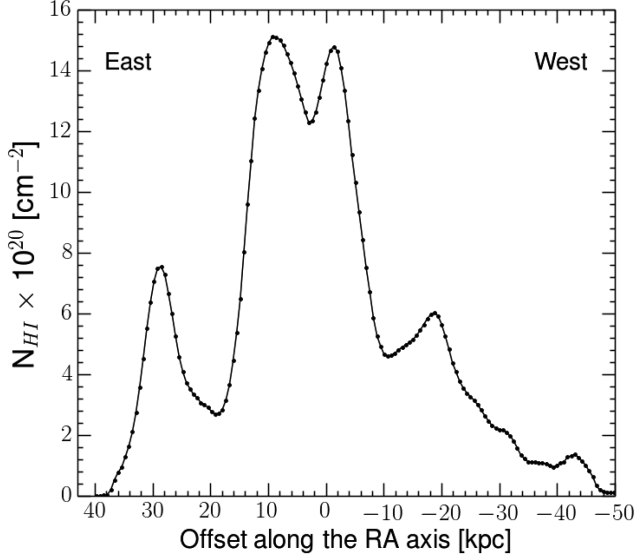
Figure 8. A column density cut across NGC 1566 with respect to right ascension offset from the centre of the galaxy. The width of this cut is 5 kpc and is shown by the blue dashed line in Fig. 7. Left-to-right in the figure corresponds to east-to-west.
