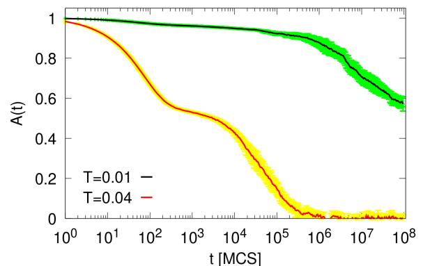
FIG. 4. Autocorrelation A(t) as a function of time t from Landau-Lifshitz dynamics at B = 0.13 in the skyrmion fluid ( T = 0.04 in red) and bimeron glass ( T = 0.01 in black). The latter is \sim 6 orders of magnitude slower than the former. Error bars are coming from averaging over different seed configurations obtained from Monte Carlo simulations.
