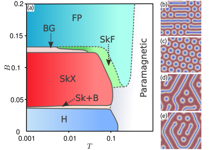
FIG. 2. (a) Phase diagram of Hamiltonian (1) at D_z = \sqrt{3} and D^\perp = 0.5 . The field-polarised (FP) phase is a resurgence of the chiral spin liquid. Thanks to its large entropy, it circles around the SkX phase at high temperature, creating an intermediate skyrmion fluid (SkF) where the density of skyrmion can be tuned with temperature. Our model further supports a “bimeron glass” (BG). Solid and dashed lines respectively indicate thermodynamic transitions and crossovers, with the caveat that simulations become glassy in the vicinity of the bimeron glass. Snapshots of spin configurations for different regions of the phase diagram: (b) the standard bimeron + skyrmion regime at B = 0.04 (Sk+B) [23], (c) the skyrmion solid at B = 0.06 and (d,e) the bimeron glass at B = 0.13 .
