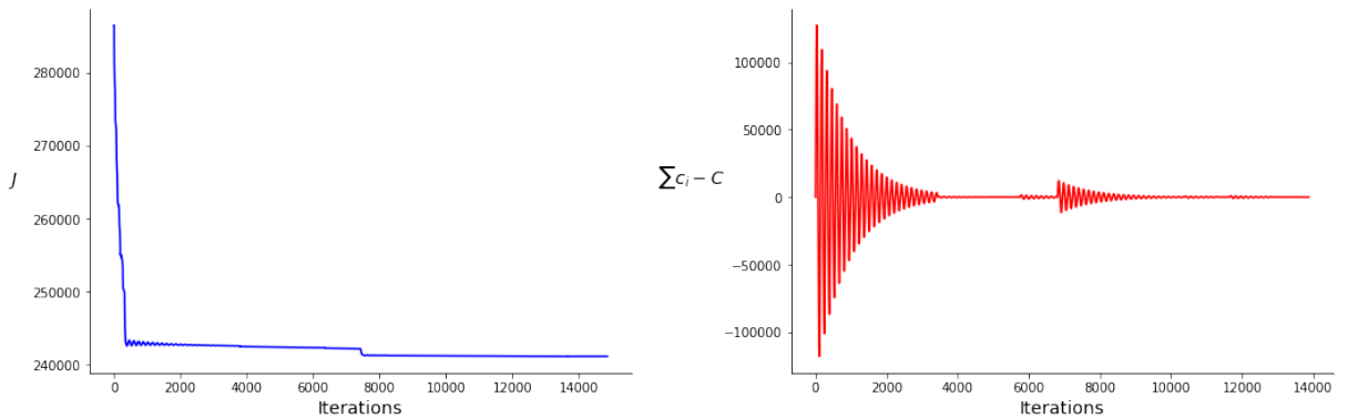
Figure 6: Evolution of the functional J(u) and \sum c_i - C during the sterile insect simulation for 20 releases and C = 3 \cdot 10^7 .
