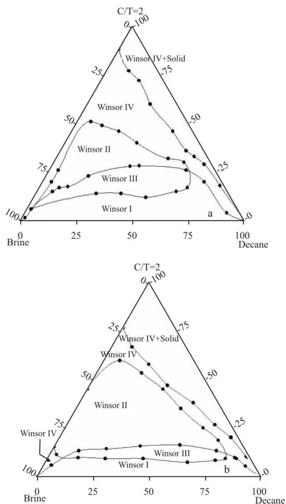
Fig. 2 Pseudoternary phase diagrams of brine/decane/surfactant-cosurfactant/systems at 30°C a – Brine/decane/sodium dodecanesulfonates butan-1-ol system; b – Brine/decane/Hostapur 60-butan-1-ol system
