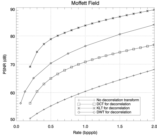
Fig. 3. Performances of the JPEG 2000 compression using either no interband decorelation, DCT, KLT, or DWT decorelation on the Moffett Field data set of Fig. 1.
