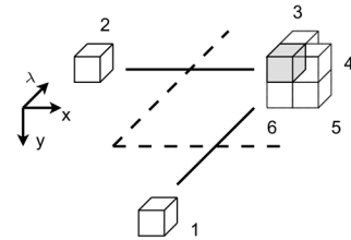
Fig. 13. Example of a tree crossing: the coefficient in grey can be considered as the spectral child of coefficient 1 together with coefficient 3 or as the spatial child of coefficient 2 together with 4, 5, and 6.
