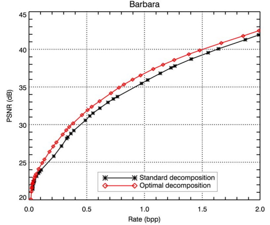
Fig. 7. Comparison between the classical decomposition and the best basis decomposition in the case of a 2-D image containing strong frequency features. For more natural images without strong frequency features, as Lena for example, the gain is negligible.
