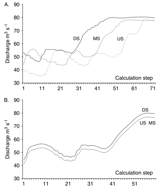
Figure 5. Discharge at each sampling point for each step of the calculation of the mass balance. US, MS and DS sampling points are represented by a dashed line, grey line and black line, respectively. (A) VRT method: one step represented half an hour only for the US site. (B) CRT method: one step represented half an hour at each site. US and MS curves are almost the same because of the low discharge variation between the sampling points
