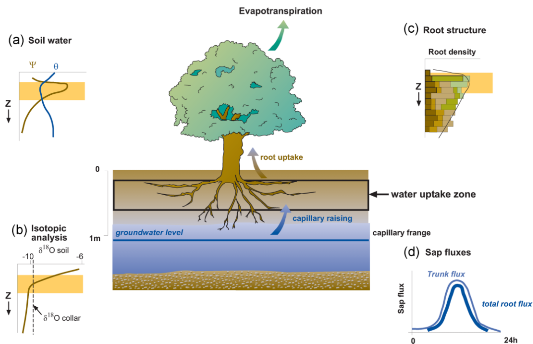
Figure 8. Scheme of water uptake by trees in the riparian forest. (a) Soil water content and water potential versus depth, (b) ^{18}\text{O} profile in the soil (dotted line shows \delta^{18}\text{O} ‰ in the trunk), (c) density of roots versus soil depth and (d) sap fluxes in trunk and root over the 24-h cycle
