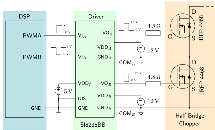
Figure 6. Schematic of the chopper
