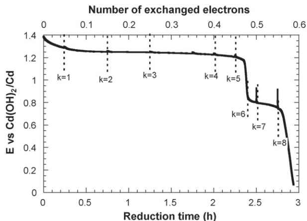
Fig. 4. Third reduction curve of a NOE electrode at C/5 rate in NaOH 5 M. At each k index an impedance electrochemical spectroscopy measurement was performed.
