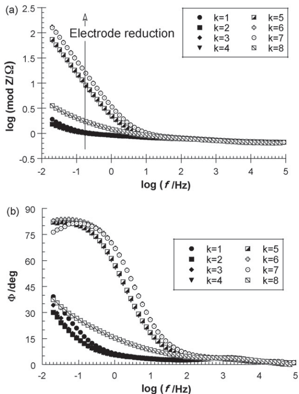
Fig. 5. Impedance modulus (a) and phase angle (b) corresponding to the measurements at different stages of reduction (see Fig. 4).
