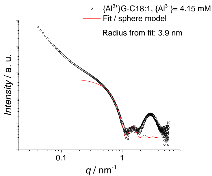
Figure S 1 – Fit of a typical SAXS profile corresponding to the \{\text{Al}^{3+}\}\text{G-C18:1} system studied in Figure 5 of the main text. The fit is performed using a simple sphere model in the software Sasview 3.1.2.
