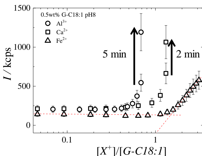
Figure 2 - Average light scattered as a function of the charge ratio [X^+]/[G-C18:1] . Arrows represent the increase of light scattered after few minutes at the same charge ratio. Intersection of dash lines correspond to the critical charge ratio of the macroscopic phase transition.
