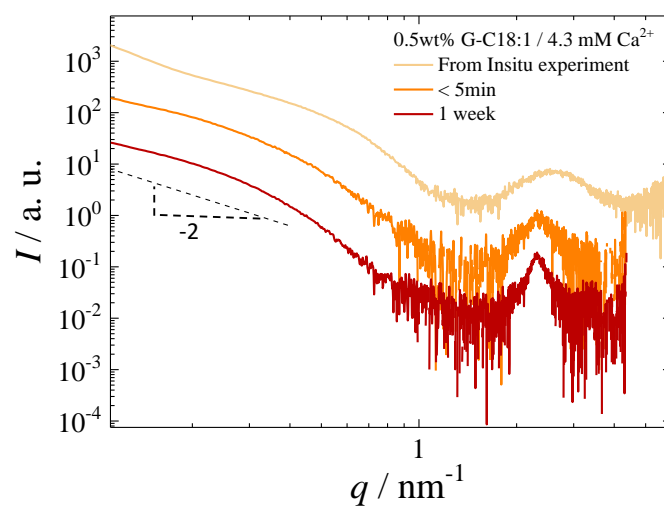
Figure S 2 – SAXS spectra of \{\text{Ca}^{2+}\} G-C18:1 solution at a molar ratio 0.4 (G-C18:1 = 0.5 wt%) at different preparation time marked in the caption.
