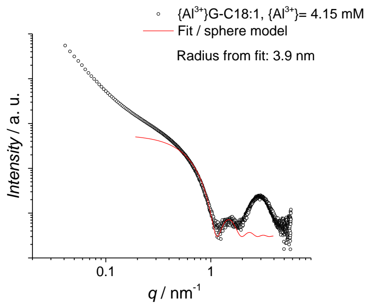
Figure S 1 – Fit of a typical SAXS profile corresponding to the {Al 3+ }G-C18:1 system studied in Figure 5 of the main text. The fit is performed using a simple sphere model in the software Sasview 3.1.2.
