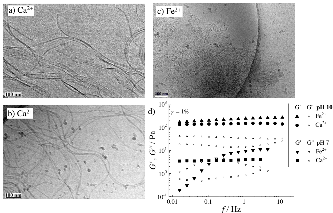
Figure 1 – Cryo TEM picture of 0.5 wt% G-C18:1 at a molecular ratio a,b) [\text{Ca}^{2+}]/[\text{G-C18:1}] = 0.61 and c) [\text{Fe}^{2+}]/[\text{G-C18:1}] = 1.4 . d) Typical frequency sweep storage (full symbols) and loss (empty symbols) moduli for calcium and iron gels ( C_{\text{G-C18:1}} = 3 \text{ wt}\% ). Spheroidal aggregates in cryo-TEM images are artefacts due to due cryo-fixation.
