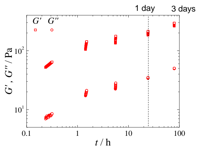
Figure S 2 – Time-dependency of the gelation ( \gamma=0.3\% , f=1 Hz) of {Ca 2+ }G-C18:1 hydrogels (C= 3 wt%, pH 10). The charge ratio is [Ca 2+ ]/[G-C18:1]= 0.61. Hydrogel is left in a closed sample-holder and sampled at regular intervals, and not left under air on the rheometer geometry.
