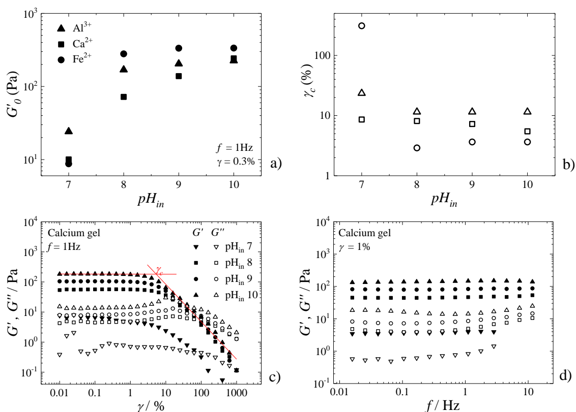
Figure 5 - a) Elastic moduli at pseudo equilibrium, G'_0 and b) critical strain, \gamma_c , of G-C18:1 hydrogels containing Ca^{2+} (square), Al^{3+} (triangle) or Fe^{2+} (circle) as a function of the initial pH, pH_{in} , of the G-C18:1 solution ( C_{G-C18:1} = 3\text{ wt\%} ) at the molar ratio [Al^{3+}]/[G-C18:1] = 0.38 , [Ca^{2+}]/[G-C18:1] = 0.61 , and [Fe^{2+}]/[G-C18:1] = 1.4 . c) Strain sweep experiment for calcium hydrogel, critical strain \gamma_c correspond to intersection of fit at linear viscoelastic domain and high strain. d) Frequency sweep experiment for calcium gel (legend in c)); curves shapes are representative of aluminium and iron derived hydrogels.
