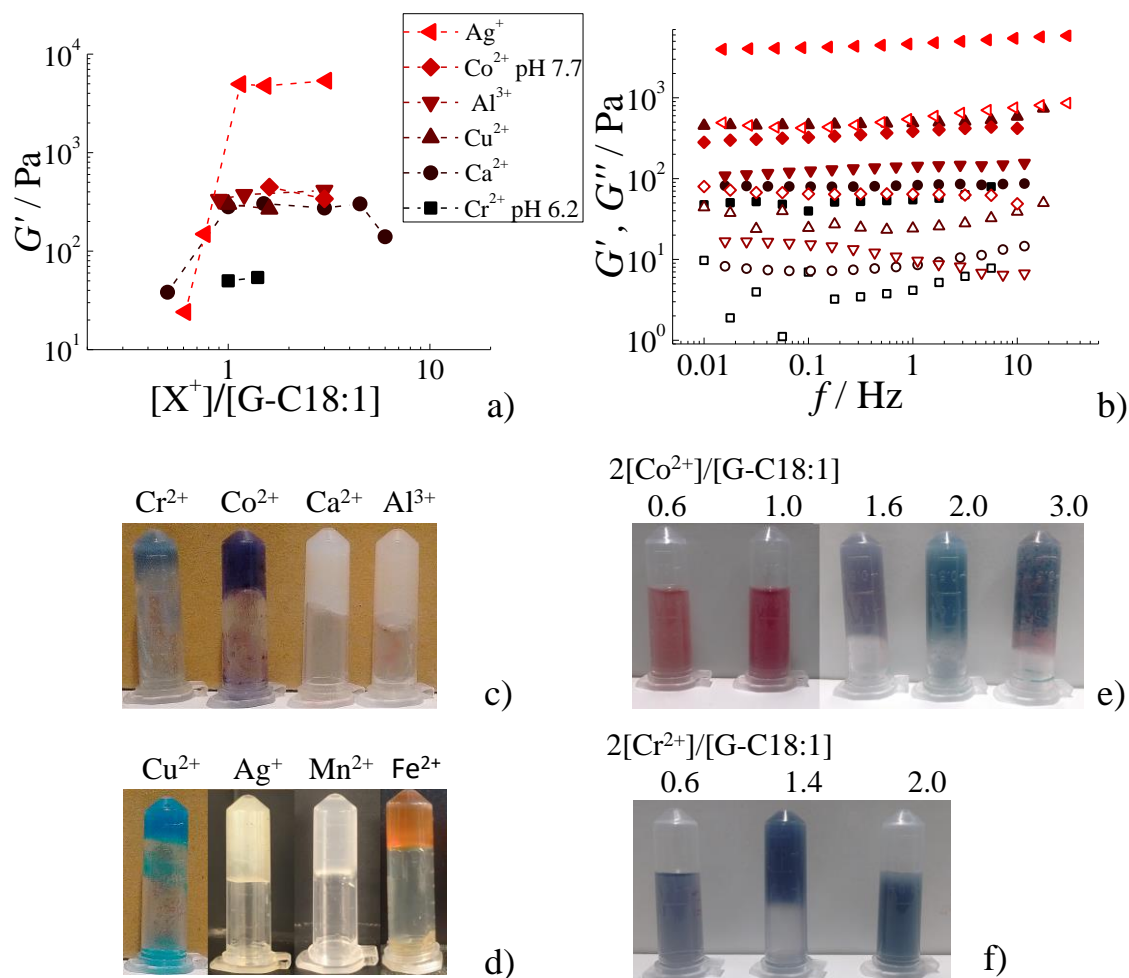
Figure 4 - a) Elastic modulus of G-C18:1 (C= 3 wt%) metallogels as a function of the charge-normalized cation molar concentration for different salts. For \text{Co}^{2+} and \text{Cr}^{2+} , the pH refers to the final manually-adjusted pH, required to obtain a gel. b) Frequency sweep measurement of the corresponding gel systems in a) at the plateau ( G' : full symbols; G'' : empty symbols). c,d) Typical images of G-C18:1 (C= 3 wt%) metallogels after about 24 h from preparation. e,f) \text{Co}^{2+} and \text{Cr}^{2+} based G-C18:1 (C= 3 wt%) metallogel freshly prepared at pH 7.7 and 6.2 for different ion-to-glucolipid charge ratio. The factor 2 in (e,f) is employed to consider the total positive charge, [X^+] (see materials and methods section).
