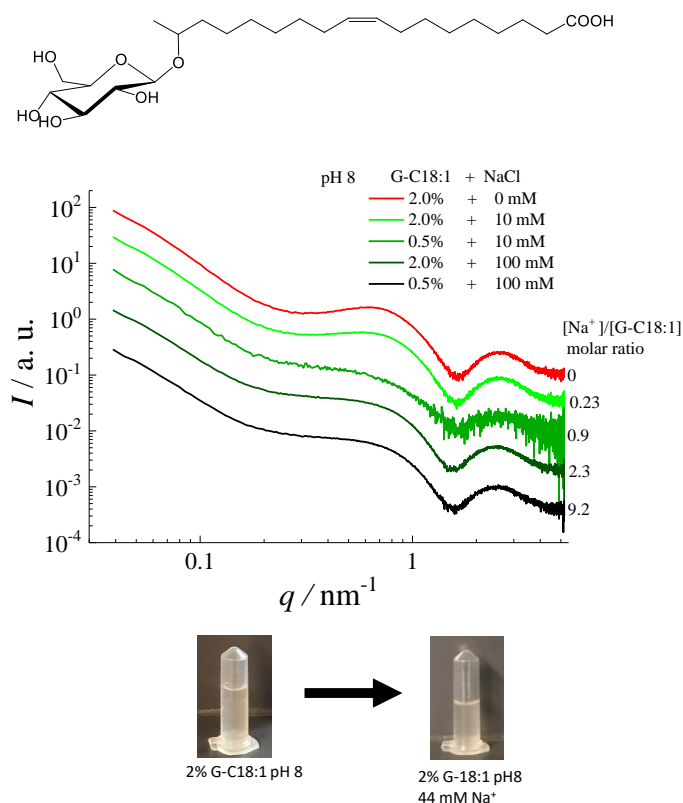
Figure 1 – SAXS spectra of a G-C18:1 microbial glucolipid solution at pH 8 and room temperature with a ratio [\text{Na}^+]:[\text{G-C18:1}] varying from 0 to 9. Concentration of G-C18:1 and NaCl are given in the figure. Concentration of 0.5 wt% and 2.0 wt% of G-C18:1 ( M_w = 460 g/mol) corresponds to 10.8 and 43.5 mM, respectively. Data have been scaled in the intensity axis by a factor five.
