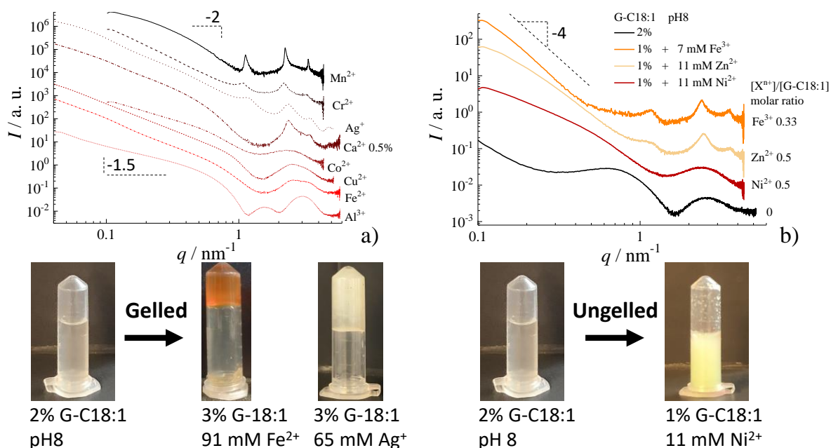
Figure 2 – SAXS profiles of a) G-C18:1 solution initially at pH 8 ( 0.5 < C / \text{wt}\% < 3 ) gelled by Mn 2+ , Cr 2+ , Ag + , Ca 2+ , Co 2+ , Cu 2+ , Fe 2+ or Al 3+ ([ion]:[G-C18:1] molar ratio vary between 0.5 and 1.5) and b) G-C18:1 aggregates containing Fe 3+ , Ni 2+ and Zn 2+ . Image of the reverse tube illustrate a typical gel in a) and aggregation in b).
