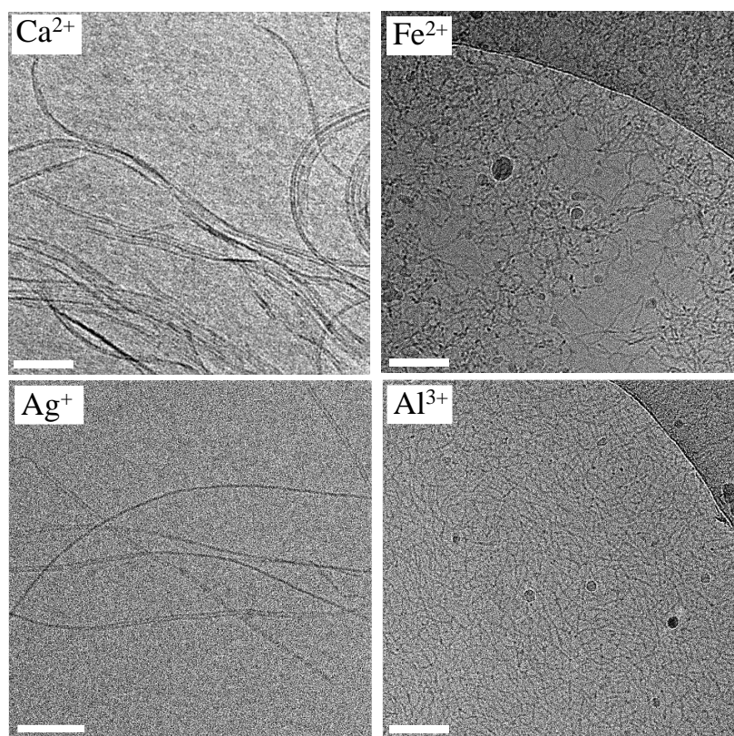
Figure 3 - Cryo TEM images of G-C18:1 solution at 0.5% (10.8 mM) containing \text{Ca}^{2+} (0.61 mM), \text{Ag}^+ (10.8 mM), \text{Fe}^{2+} (16 mM) and \text{Al}^{3+} (0.34 mM). Additional cryo-TEM images are provided in Figure S 1 in the Supporting Information. The spheroidal aggregates spuriously observed in \text{Fe}^{2+} and \text{Al}^{3+} images are typical artefacts due to cryo-fixation. 57 Scale bar is 100 nm for all images.
