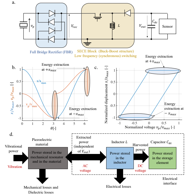
Figure 3. a. System implementation, b. normalized transient waveforms, c. (x v_p) cycle of a CDE strategy (SECE), and d. power flow of a CDE strategy (SECE).
