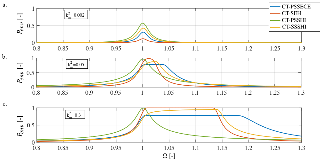
Figure 16. Harvested power envelopes of the CT-PSSECE (blue), CT-SEH (red), CT-SSHI (yellow), and CT-PSSHI (green), with Q_m = 50 , \beta_{min} = -0.8 and a. k_m^2 = 0.002 b. k_m^2 = 0.05 c. k_m^2 = 0.3
