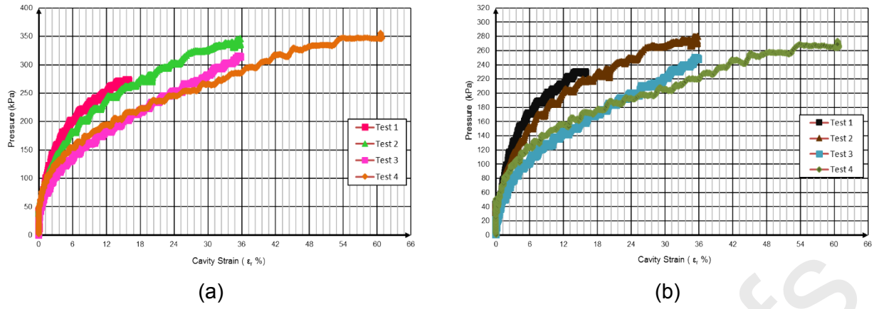
Fig. 20. Results of monotonic tests on dense sand. (a) raw curves; (b) corrected curves
