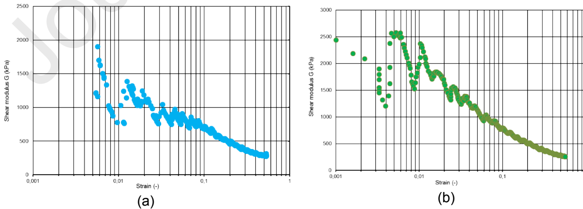
Fig. 19. Evolution of the shear moduli G with the cavity strain. (a) Test 1, (b) Test 3
