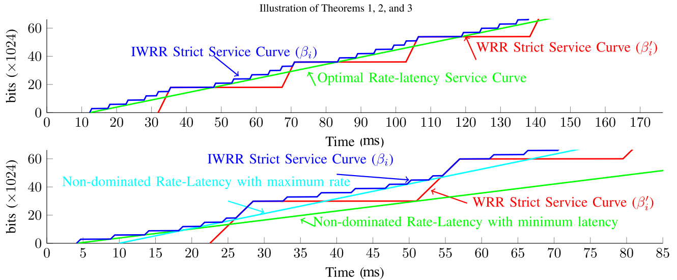
Fig. 3 Strict service curves obtained in Sect. 5 for an example with four input flows, weights = {4, 6, 7, 10}, l^{\min} = \{4096, 3072, 4608, 3072\} bits, l^{\max} = \{8704, 5632, 6656, 8192\} bits and \beta(t) = ct with c = 10 Mb/s (i.e., the aggregate of all flows is served at a constant rate). The figure shows the IWRR service curve \beta_i and the WRR strict service curve \beta'_i for two of the flows; it also shows the non-dominated rate-latency strict service curves \beta_{r_0^*, T_0^*} and \beta_{r_k^*, T_k^*} of Theorem 3 (in the top panel both are equal).
