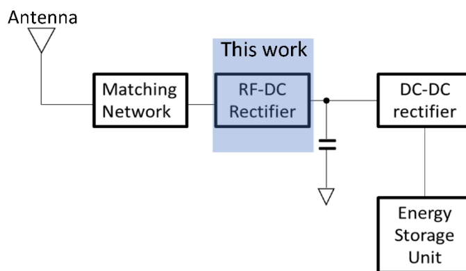
Figure 1. RF Energy Harvesting (RFEH) system description and specific focus on the rectification or RF-DC conversion stage that is the focus of this work.
