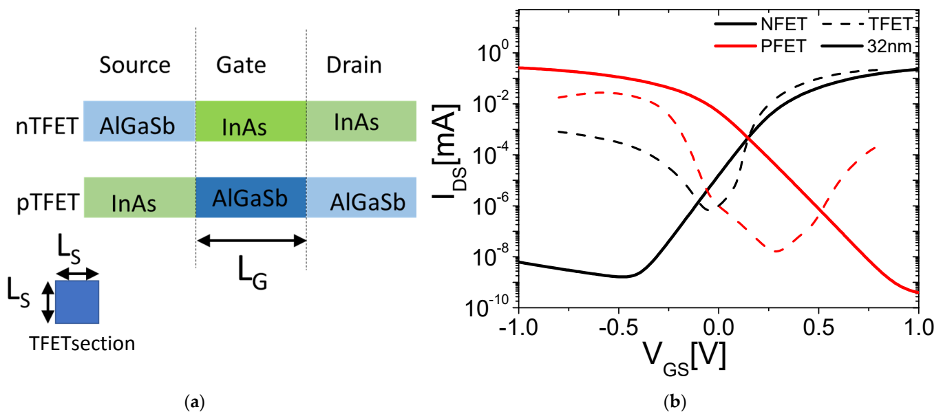
Figure 2. (a) Nanowire (NW) structure of the considered TFET. The NW section is a square of side L_S = 7 nm. The gate length is L_G = 20 nm, and the gate dielectric consists of 2.3 nm of Al_2O_3 all around the gate portion, which results in an EOT = 1 nm; not shown. (b) The simulation of I-V characteristics of the 32 nm MOSFET and the Tunnel-FET for p- and n-FET.
