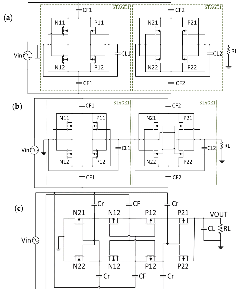
Figure 3. Different CCDD-based topologies used in this work: (a) conventional CCDD or CDC (only TFET), (b) conventional/body bias or CDB (only for 32 nm), and (c) bias control by level shift or CDC (32 nm and TFET). Note that CDN is not a cascaded configuration as in the topology CDC and CDB.
