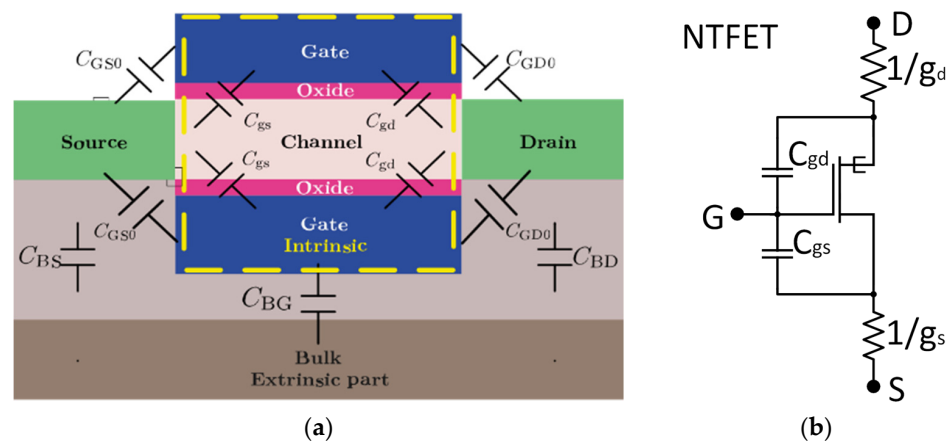
Figure 6. Description of the model used for the parasitic components of the TFET: (a) the capacitive contribution related to the TFET architecture (transversal cut) considered based on the model in [22], (b) the electrical circuit model resulting from the capacitive parasitic components.
