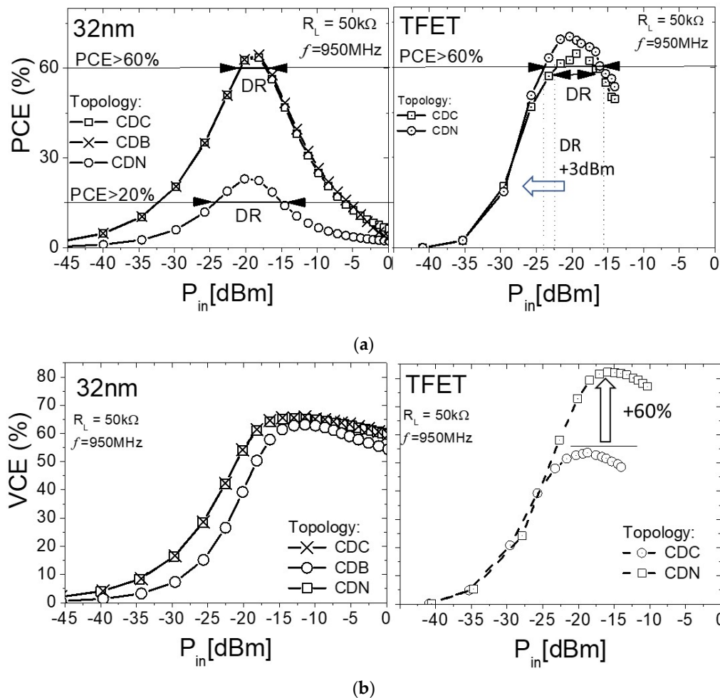
Figure 7. The FOM to assess the performance of the different topologies for different technology: (a) the PCE and (b) the VCE. In (a), the PCE for the TFET is the DR (>60%), which is increased from 5 dBm to 8 dBm or 3 \mu W to 6 \mu W. For the 32 nm, the DR is not improved if we use the back bias to control the V_{TH} (CDB circuit). The PCE is importantly degraded for the CDN topology with 32 nm.
