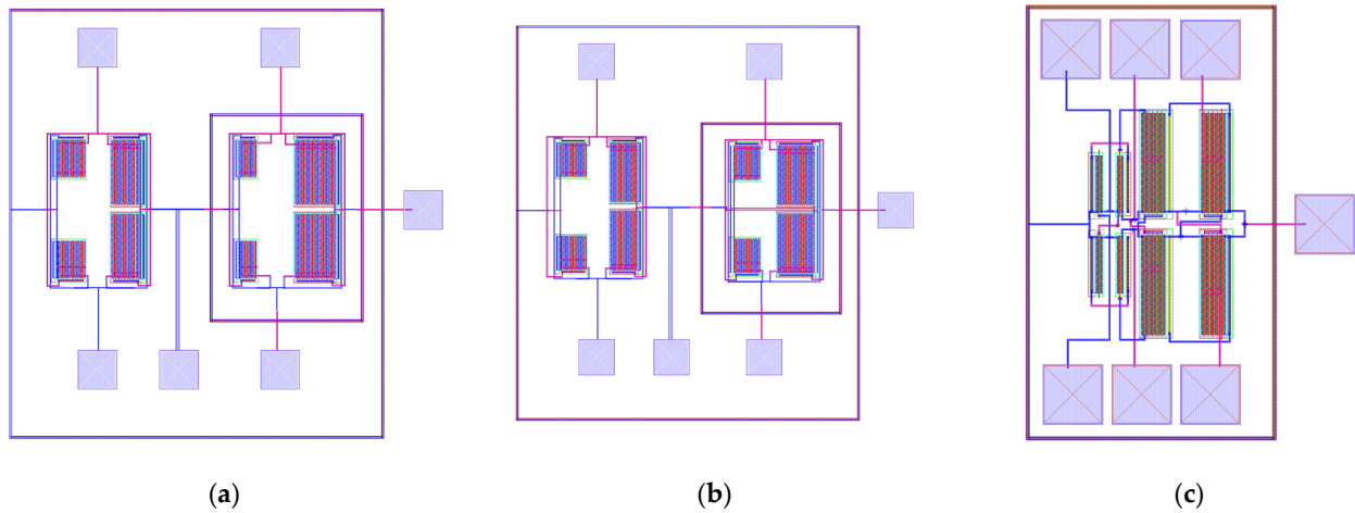
Figure 5. Layout of the topology CDC (a), CDB, (b) and CDN (c) in 32 nm with, the iPDK using Cdesigner. The capacitors are not represented because they are occupying much more space in the layout. In practice, the large capacitors can be used in the metal layers.
