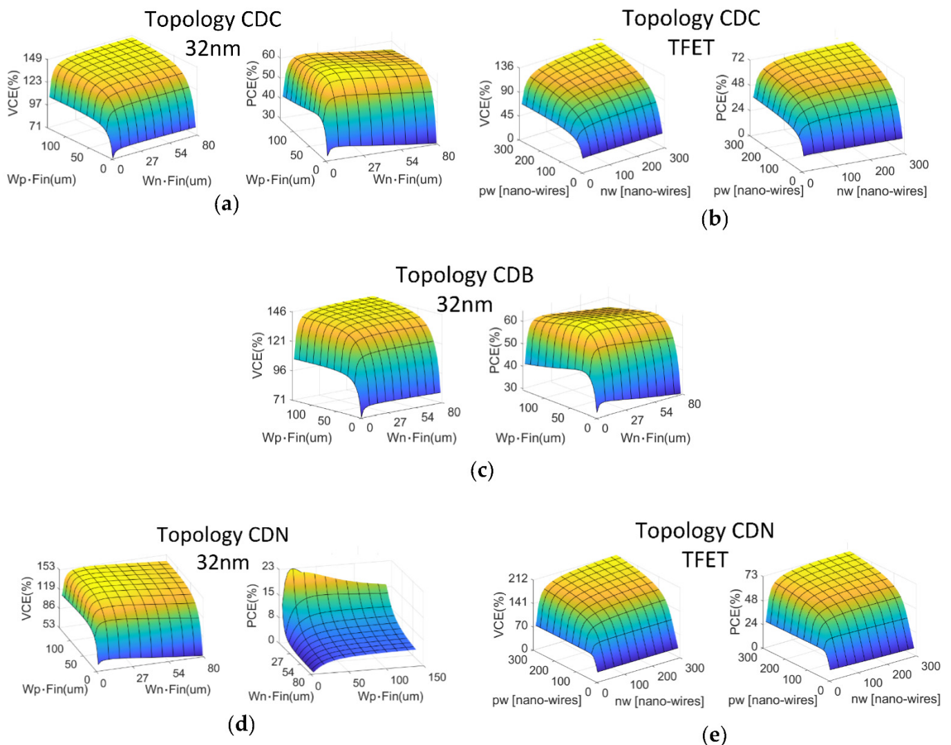
Figure 4. VCE and PCE optimization for circuit sizing of the different CCDD-based topologies studied in this work: (a,b) the conventional topologies [Figure 4a] in 32 nm and TFET, respectively; (c) the first stage is conventional and the second stage is body bias [Figure 4b] with only 32 nm technology; (d,e) two-stage with bias level shift in the second stage [Figure 4c] for 32 nm and TFET techno, respectively. The load is fixed to 50 k \Omega and L_n = L_p = 30 nm for the 32 nm technology. For the TFET, see the details in Figure 2.
