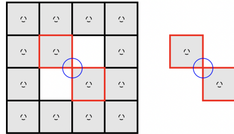
Fig. 19: When X contains a critical configuration \{p, p'\} of center m , the boundary of \text{CA}(X) behaves like the union of the boundaries of the continuous analogs of p and p' in the neighborhood of m (see the part of the red self-crossing curve included in the blue circle). [This picture is better viewed in colour.]
