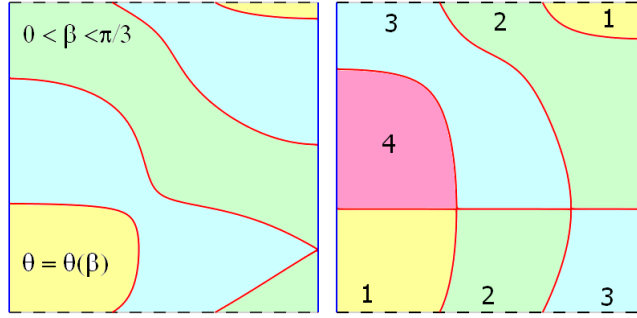
FIGURE 4.3. Partition associated with eigenfunctions of the Möbius strip
