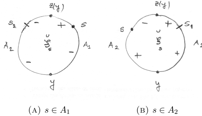
FIGURE 9.9. Signs of the function \check{\xi}_s
