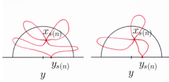
FIGURE 9.5. Proof of Lemma 9.2: Case C2i, forbidden configurations
