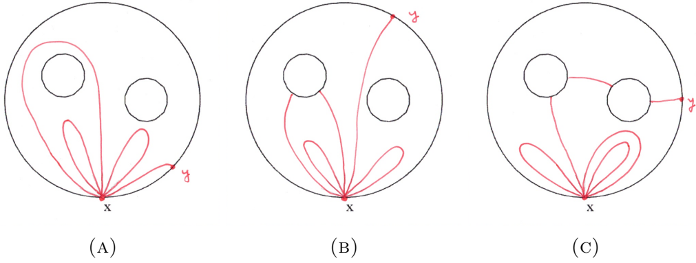
FIGURE 7.4. \Omega with two holes: some possible nodal patterns for u_{x,y}
