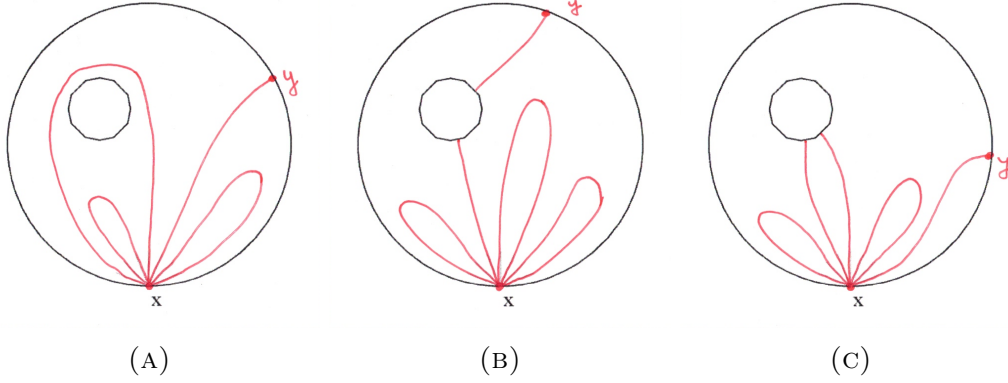
FIGURE 7.2. \Omega with one hole: some possible nodal patterns for u_{x,y}
