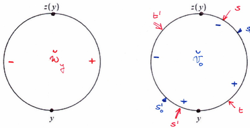
FIGURE 9.18. Proof of Lemma 9.13(i)
