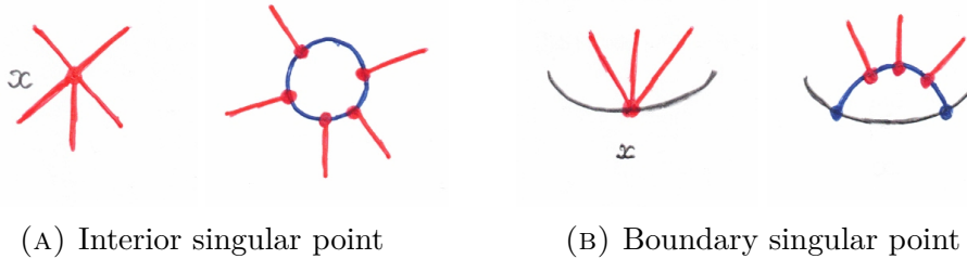
FIGURE 4.1. Normalization at a singular point
