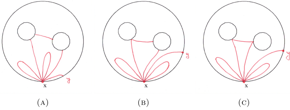
FIGURE 7.5. \Omega with two holes: some possible nodal patterns for u_{x,y}
