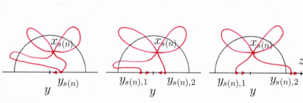
FIGURE 9.4. Proof of Lemma 9.2: Case C2, nodal patterns
