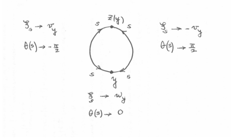
FIGURE 9.11. Lemma 9.8: limits of \xi_s when s tends to y or z(y)
