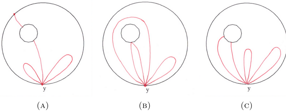
FIGURE 8.4. \Omega with one hole, some nodal patterns for w_y
