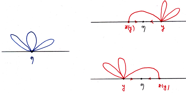
FIGURE 10.5. The combinatorial types of Z(w_y) are different on the right and on the left of \eta \in \Gamma_{(2k-2)}
