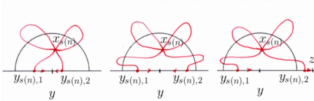
FIGURE 9.6. Proof of Lemma 9.2: Case C2, forbidden configurations
