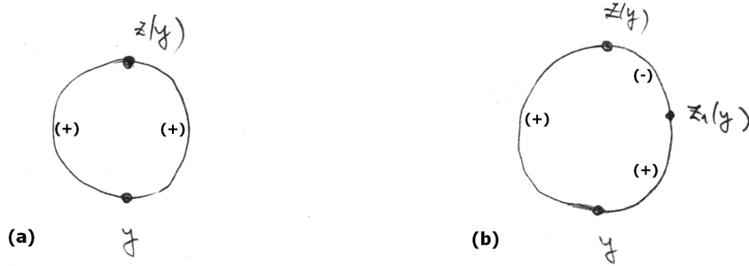
FIGURE 9.7. Signs of \check{v}_y , Cases (a) and (b)
