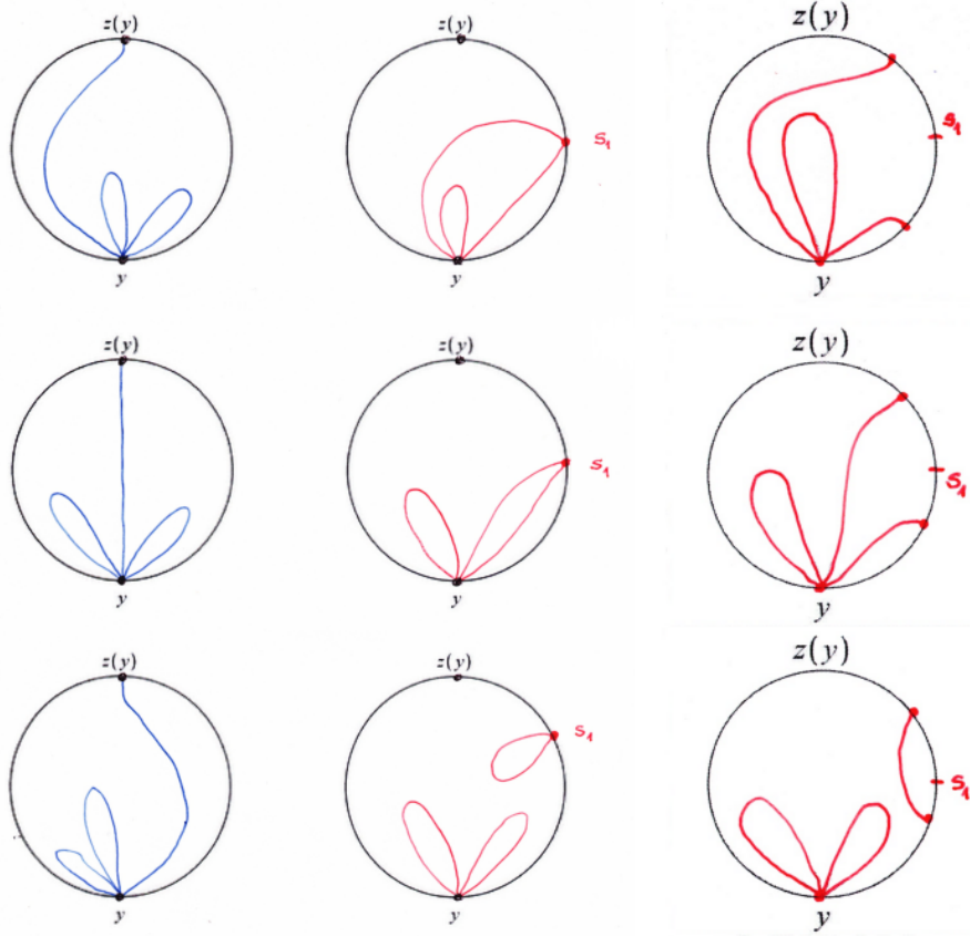
FIGURE 9.22. Lemma 9.13 (ii) and (iii): nodal patterns for w_y and v_{y,s_1}
