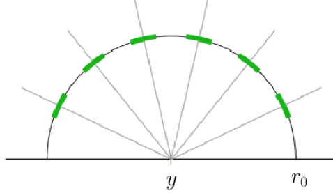
FIGURE 9.1. Proof of Lemma 9.2: the set C^+(r_0, w, \varepsilon_1)
