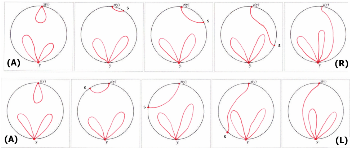
FIGURE 9.13. The point s tends to y clockwise (top) or counter-clockwise (bottom), here k = 4
