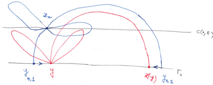
FIGURE 10.1. \mathcal{Z}(u_n) (blue) and \mathcal{Z}(w_y) (red)
