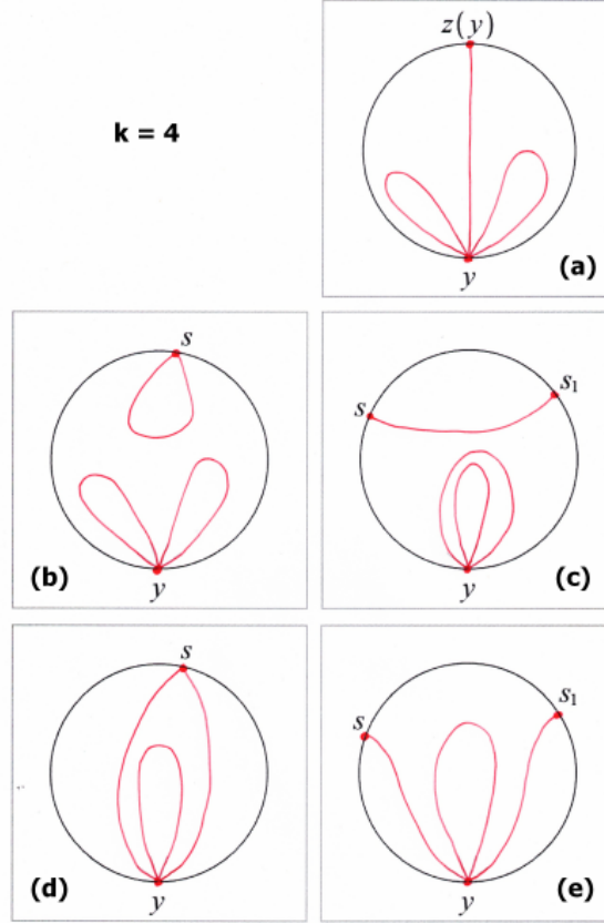
FIGURE 9.15. Nodal patterns for u \in V_{y,s} ( k=4 )
