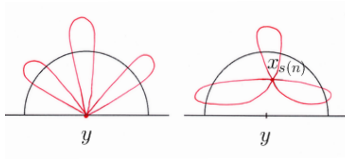
FIGURE 9.2. Proof of Lemma 9.2: Case C1, nodal pattern.
