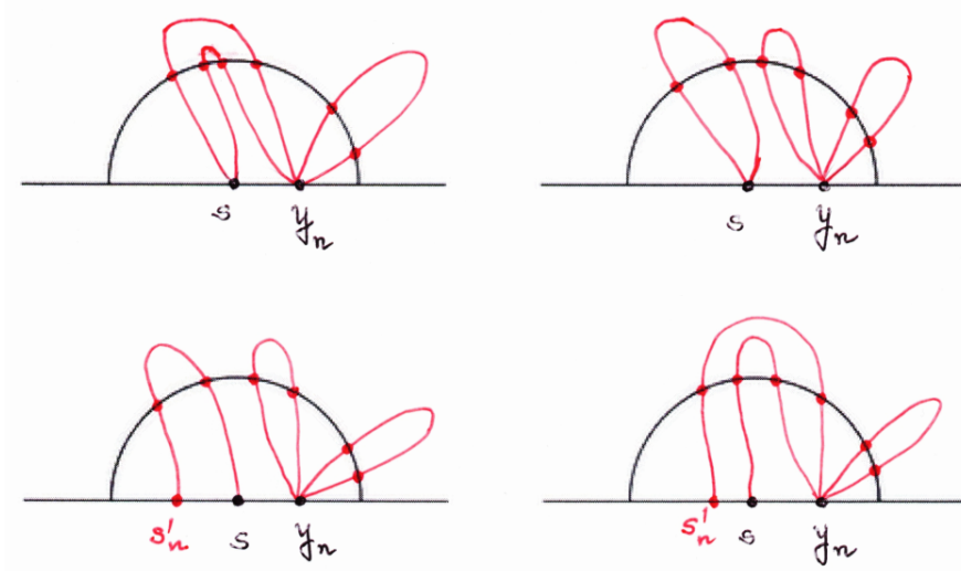
FIGURE 9.16. Proof of Lemma 9.11(iv)
