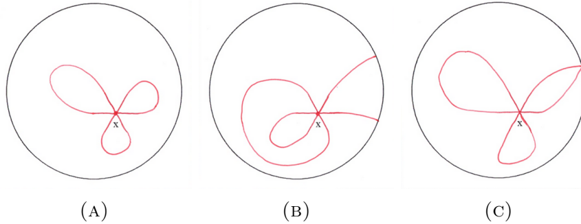
FIGURE 8.1. \Omega simply connected, some nodal patterns for u_x
