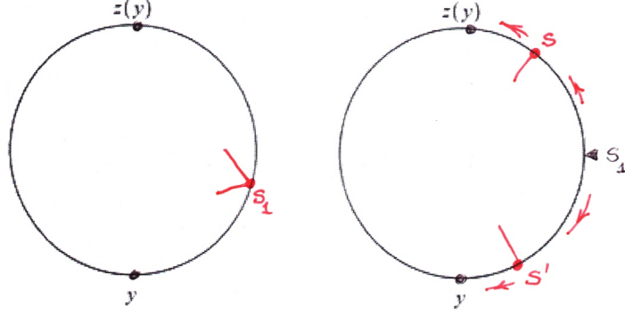
FIGURE 9.17. Lemma 9.13: Assertions (ii) and (iii)
