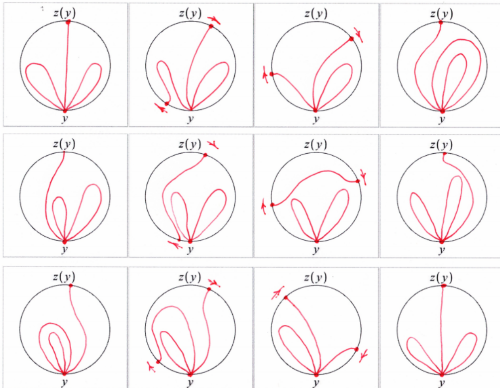
FIGURE 9.19. Proof of Lemma 9.13(i)
