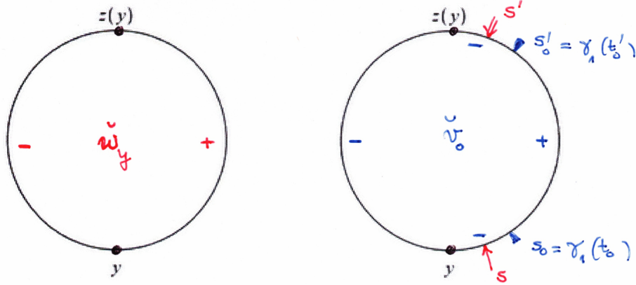
FIGURE 9.20. Proof of Lemma 9.13(ii)
