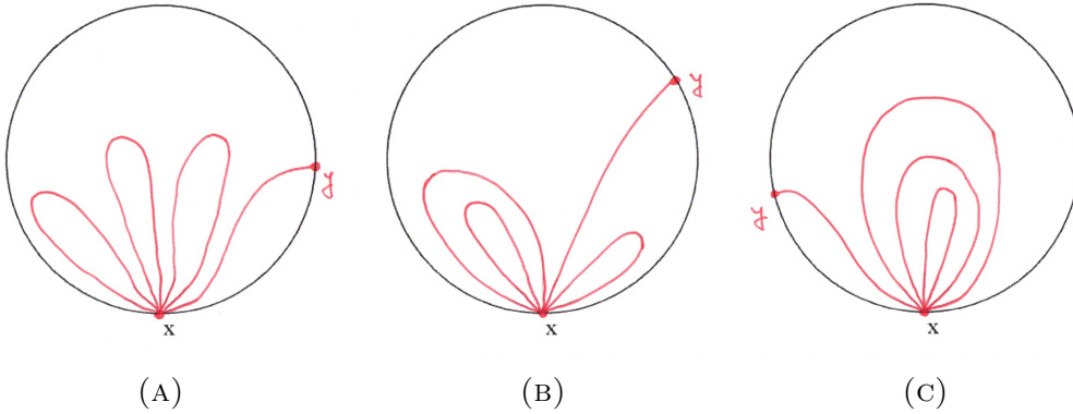
FIGURE 7.1. \Omega simply connected: some possible nodal patterns for u_{x,y}
