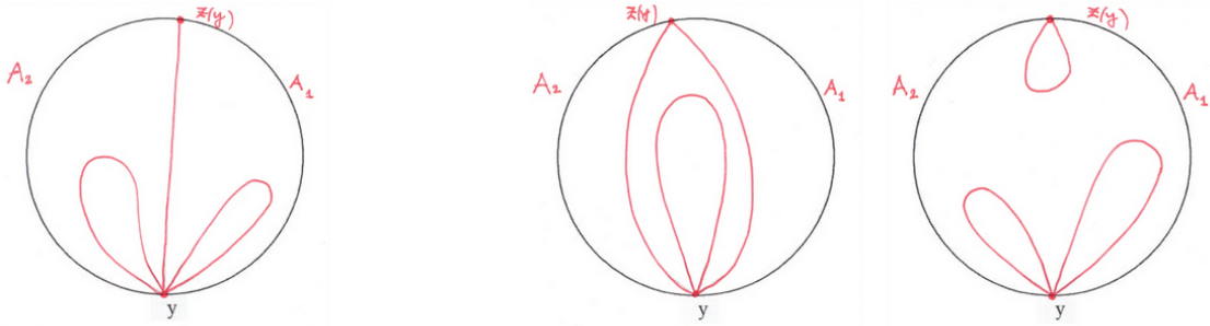
FIGURE 9.8. Nodal sets of w_y (left) and v_y (right), with k = 4 .
