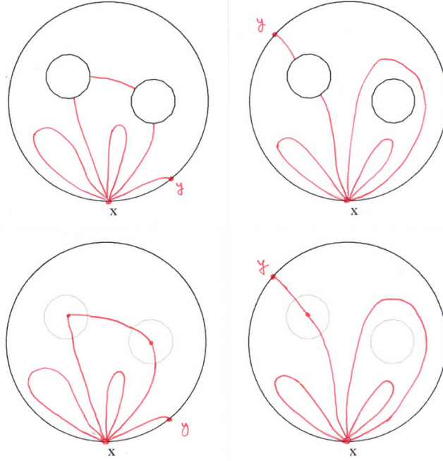
FIGURE 7.6. Nodal patterns in \Omega and their projections in \check{\Omega}
