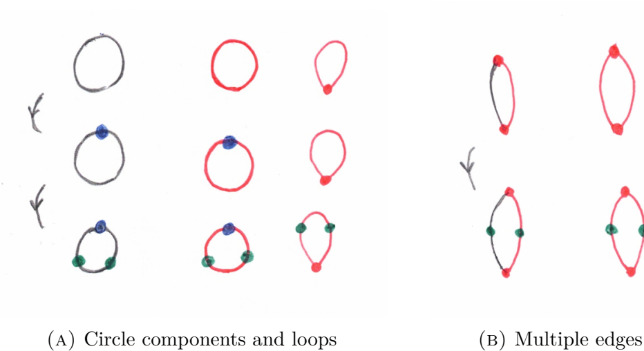
FIGURE 4.2. Vertex-edge additions
