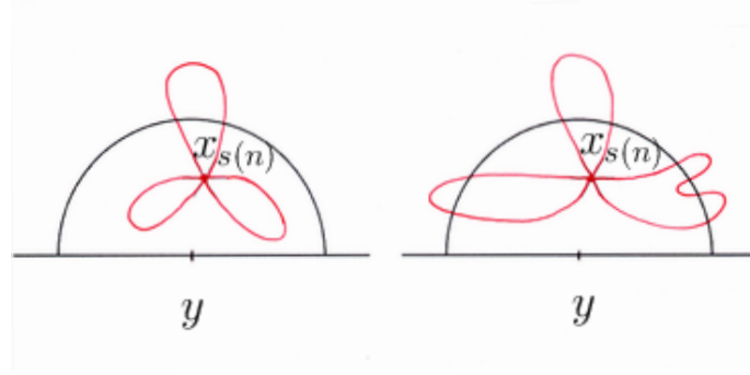
FIGURE 9.3. Proof of Lemma 9.2: Case C1, forbidden configurations.
