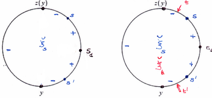
FIGURE 9.21. Proof of Lemma 9.13, Assertion (iii)
