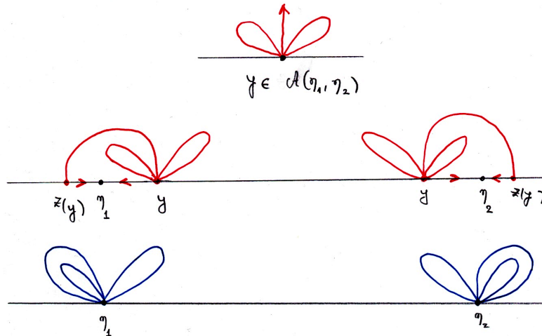
FIGURE 10.4. Z(w_{\eta_1}) and Z(w_{\eta_2}) have different combinatorial types
