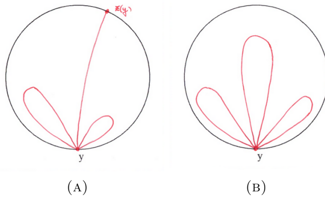
FIGURE 8.3. \Omega simply connected, some nodal patterns for w_y
