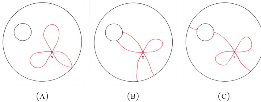
FIGURE 8.2. \Omega with one hole, some nodal patterns for u_x
