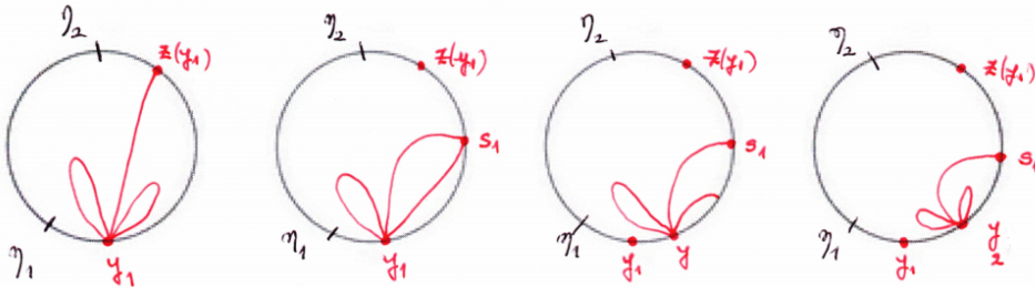
FIGURE 10.2. 1st possibility
