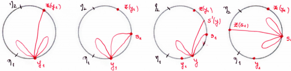
FIGURE 10.3. 2nd possibility: apparent counterexample to the claim on the nodal type
