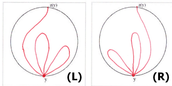
FIGURE 9.14. The nodal patterns (L) and (R) are different
