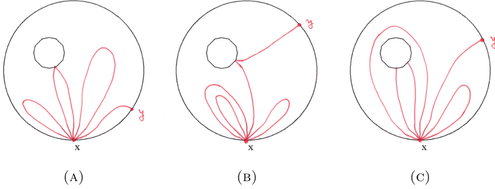
FIGURE 7.3. \Omega with one hole: some possible nodal patterns for u_{x,y}
