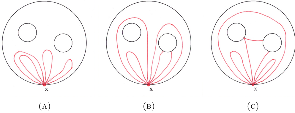
FIGURE 7.7. Some possible nodal patterns for 0 \neq u \in U_x^1
