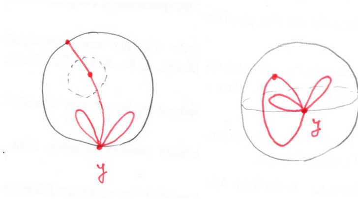
FIGURE 8.5. Figure 8.4 viewed in \check{\Omega} (left) or in \mathbb{S}^2 (right)
