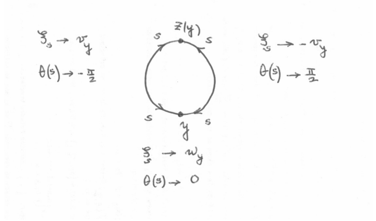
FIGURE 9.11. Lemma 9.8: limits of \xi_s when s tends to y or z(y)
