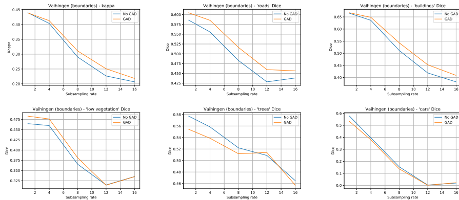
Fig. 19 Results for improving segmentation boundaries on the Vaihingen dataset considering only pixels around region boundaries. The effect of postprocessing results with GAD becomes clearer where one semantic region encounters another.
