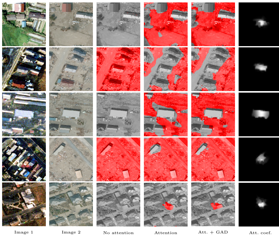
Fig. 14 Results obtained by using the proposed method. Note that when the attention layer is not used, the network does not learn to localize the features and tends to predict all pixels into the same class. The attention layer enables the network to localize features much more accurately, and the GAD post-processing further increases the spatial accuracy of such predictions. Changes are marked in red.
