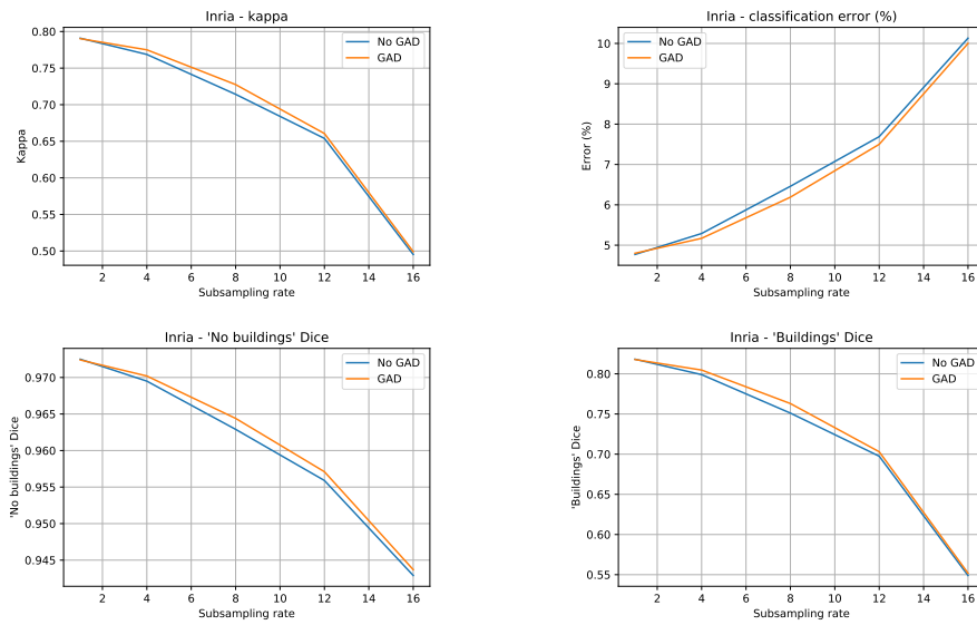
Fig. 16 Results for improving segmentation boundaries on the Inria Aerial Image Labeling Dataset. Consistent improvements across all metrics have been observed for all subsampling rates bigger than 1.
