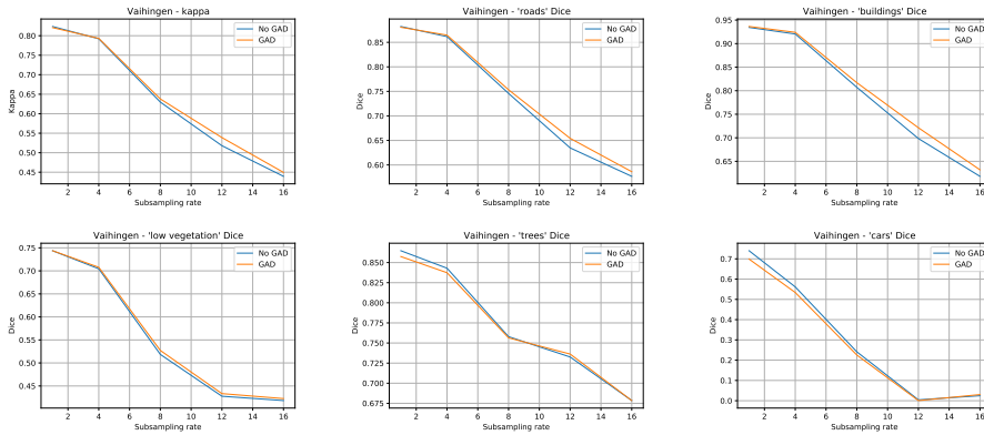
Fig. 18 Results for improving semantic segmentation on the Vaihingen dataset. Using GAD to postprocess the outputs consistently improves results for classes with larger objects and sharp visible edges.
