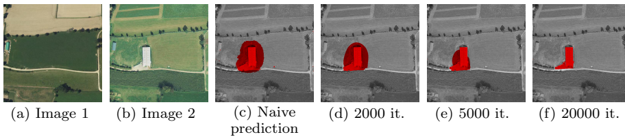
Fig. 8 Guided anisotropic diffusion for filtering a real example of semantic segmentation. The diffusion allows edges from the guide images to be transferred to the target image, improving the results (change area in red).
