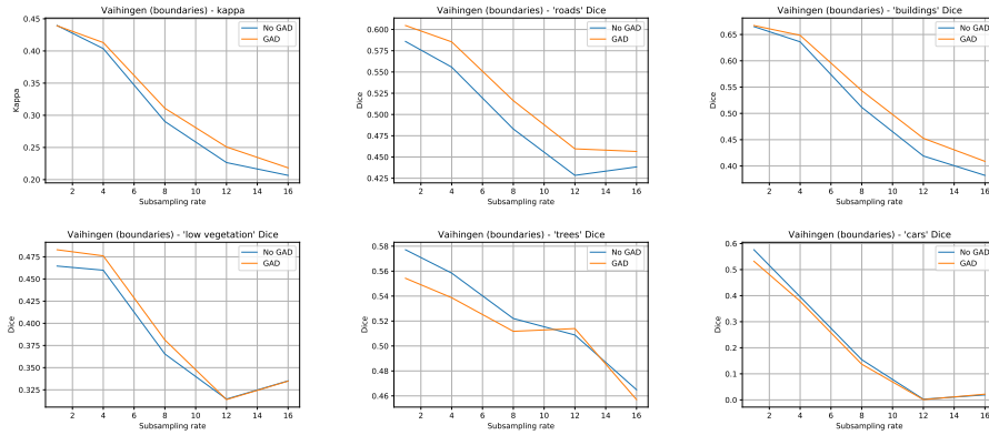
Fig. 19 Results for improving segmentation boundaries on the Vaihingen dataset considering only pixels around region boundaries. The effect of postprocessing results with GAD becomes clearer where one semantic region encounters another.
