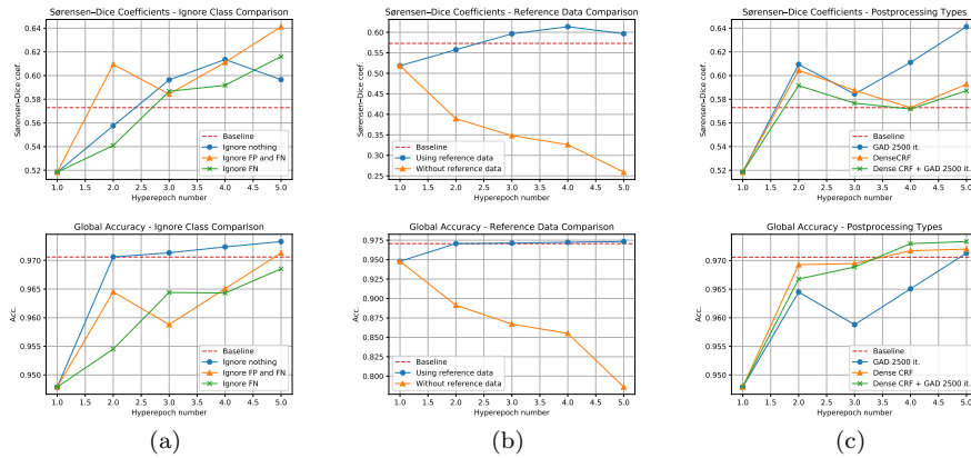
Fig. 10 Ablation studies. (a) Comparison between strategies for merging network predictions and reference data. (b) Comparison between iterative training with and without the usage of original reference data. (c) Comparison between GAD and Dense CRF. Top row contains Dice scores, bottom row contains global accuracy curves.
