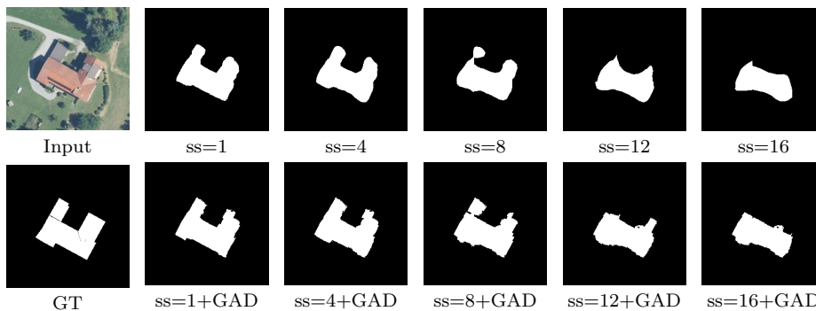
Fig. 15 Results obtained from experiments on the Inria Aerial Image Labeling Dataset. GAD successfully mitigated the accuracy loss in region boundaries at higher subsampling rates.
