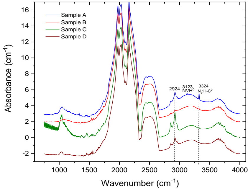
Fig 2. FTIR spectra of different freestanding CVD diamond plates grown with \text{N}_2\text{O} addition after electron irradiation and thermal annealing. The spectra were normalized to the 2-phonon absorption at around 2000 \text{cm}^{-1} and vertically shifted for clarity.
