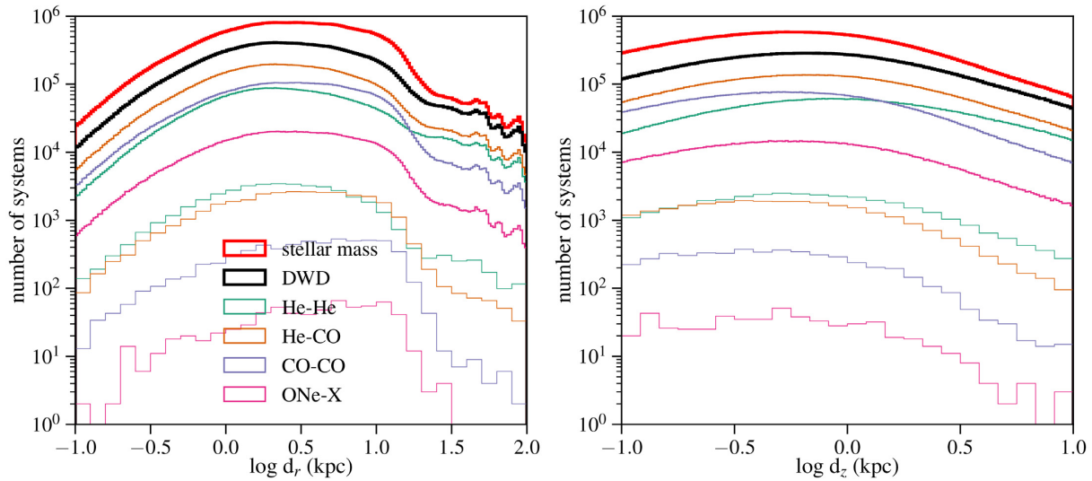
Figure 4. Spatial distributions of the DWDs (black) in comparison with the stellar mass (red, rescaled by a factor 1000). Different colours show different subtypes, and the thin lines only show the binaries with f_{\text{GW}} > 10^{-3} Hz. Both plots have the same legend.
