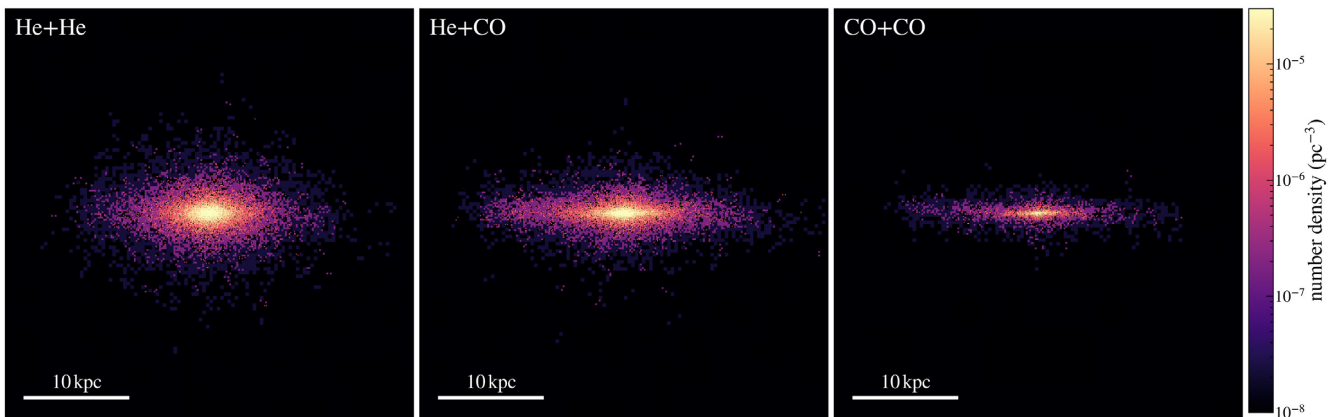
Figure 5. Maps of the He–He DWDs (left), He–CO (middle), and CO–CO DWDs (right) viewed edge-on. These maps only show the binaries with f_{\text{GW}} > 10^{-3} Hz, which are the most likely to be individually resolved by LISA . We do not show the Ne + X binaries due to their sparsity. Their distribution is very similar to the COCO binaries.
