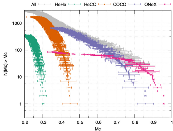
Figure 11. Number of binaries above a given chirp mass, with a well measured chirp mass, for each binary subtype. Each point shows an individual systems with chirp mass errors below 10 per cent, shown with the error bar. For this simulation (8 yr observing time) we can expect to unambiguously identify O(1000) He–CO DWDs, O(300) CO–CO DWDs, and O(10) ONe–X systems.
