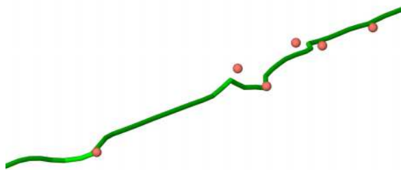
FIG. 4. Dislocation line (green) adopting a complex three-dimensional kinked structure in presence of carbon atoms (red spheres). Only the solutes closest to the dislocation are represented for clarity. The dislocation line was identified using the DXA algorithm [74].
