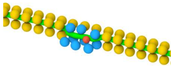
FIG. 6. Local conversion of the screw dislocation core during a dynamical simulation. The smaller red atom is a carbon atom, while all others are iron atoms. Iron atoms that adopt a distorted prismatic structure near the carbon atom, are highlighted in blue. The dislocation line obtained using the DXA algorithm is shown in green. For clarity, only core atoms are shown.
