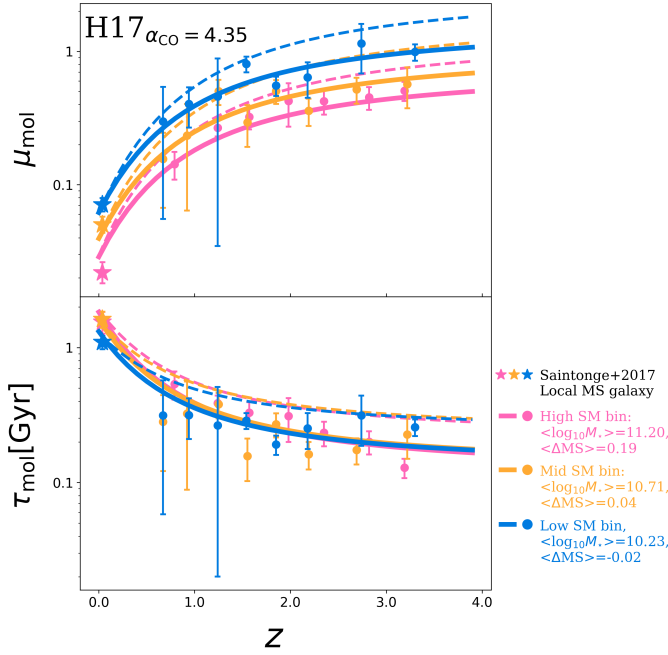
Fig. B.2. Redshift evolution of the mean molecular gas fraction and molecular gas depletion time of MS galaxies, with the M_{\text{gas}} from the \text{H17}_{\alpha\text{CO}=4.35} gas mass calibration. Dots show the mean molecular gas fraction and molecular gas depletion time from our work. Stars represent the local reference taken from Saintonge et al. (2017). Solid lines display the analytical evolution of the molecular gas fraction and molecular gas depletion time inferred with the \text{H17}_{\alpha\text{CO}=4.35} gas mass calibration. Dashed lines show the analytical evolution of the molecular gas fraction and molecular gas depletion time inferred with the H17 gas mass calibration (used throughout the paper). Symbols and lines are color-coded by stellar mass.
