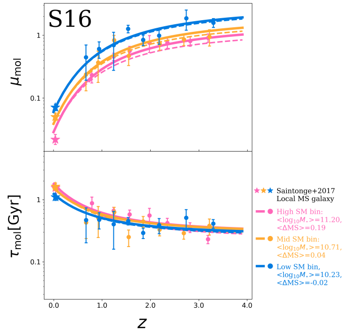
Fig. B.3. Same as Fig. B.2 but for the gas mass calibration from S16.
