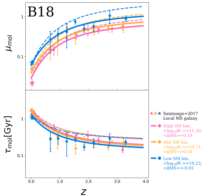
Fig. B.4. Same as Fig. B.2 but for the gas mass calibration from B18.
