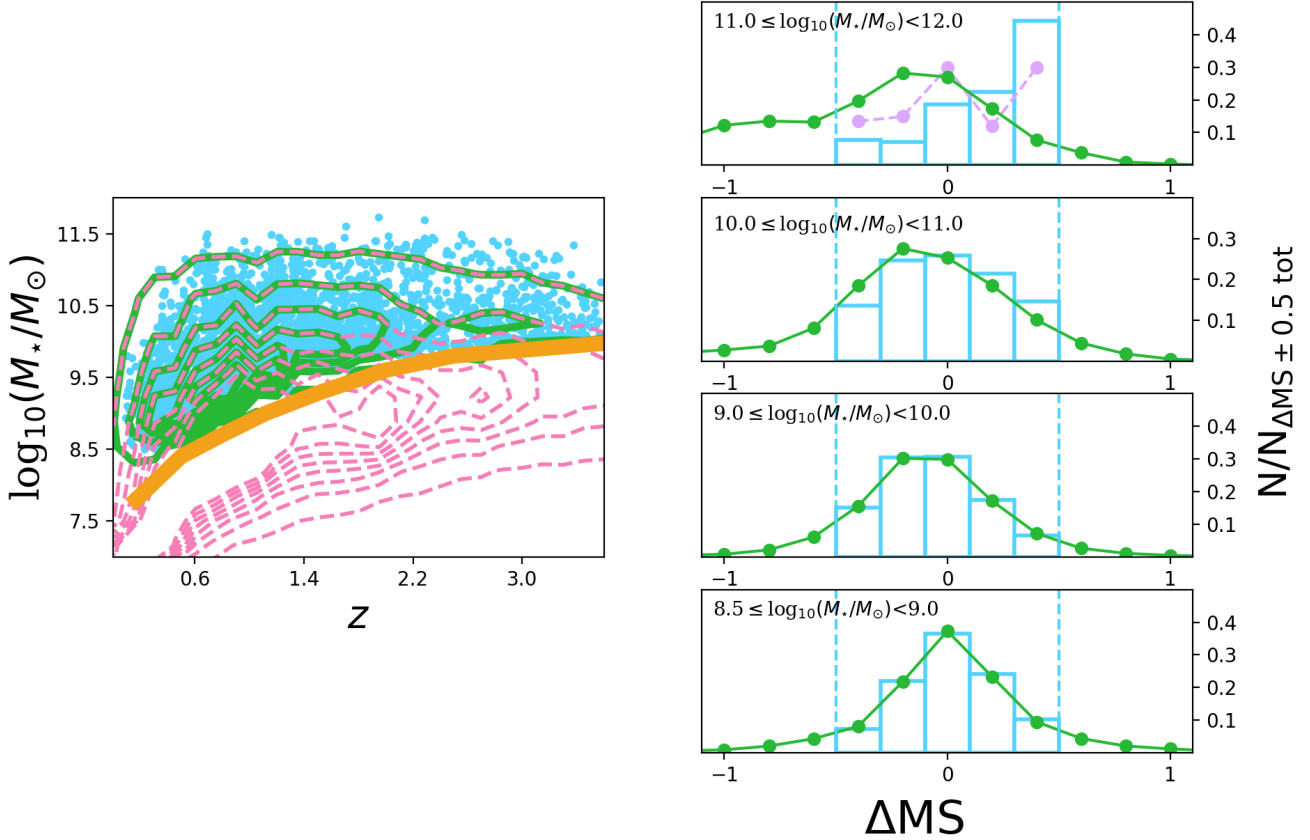
Fig. 1. Completeness and relative \Delta\text{MS} distribution in our final sample. Left: Stellar mass and redshift distribution in our final ALMA-covered mass-complete sample of MS galaxies (blue dots). The dashed pink contours display the number density of SFGs in Laigle et al. (2016), i.e., our parent sample of SFGs. The pink contour levels are in steps of 500 from 200 to 3700 galaxies per z - \log_{10} M_* bin of size 0.14 and 0.15, respectively. The solid orange line represents the stellar mass completeness limit of SFGs in Laigle et al. (2016). The green contour shows the number density of SFGs in Laigle et al. (2016) above this stellar mass completeness limit, i.e., our parent mass-complete sample. The green contour levels are in steps of 500 from 200 to 3700 galaxies per z - \log_{10} M_* bin of size 0.14 and 0.15, respectively. Right: Relative \Delta\text{MS} distribution in our final ALMA-covered mass-complete sample of MS galaxies (blue histogram) and our mass-complete parent sample of SFGs (green histogram) in different stellar mass bins. In the highest stellar mass bin, the dashed purple line shows the relative \Delta\text{MS} distribution after having rejected from our final sample all ALMA primary targets, i.e., galaxies at the phase center of the ALMA observation. The vertical dashed blue lines display the \pm 0.5 dex interval used to defined MS galaxies. Over this interval, the integral of each histogram is equal to one. This normalization is needed to compare our final and mass-complete parent samples, which contain 3037 and 515 465 galaxies, respectively.
