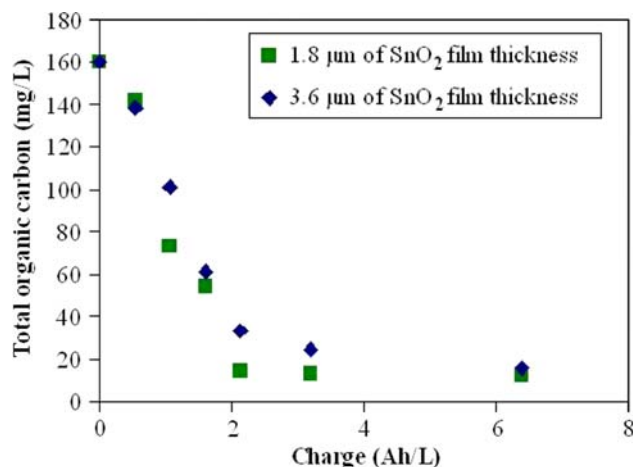
Fig. 10 Variation of TOC of electrolyze during mineralization using \text{SnO}_2/\text{Ir}/\text{Ti} , electrode surface area of 3.2 \text{ cm}^2 and current density of 5 \text{ mA}/\text{cm}^2
