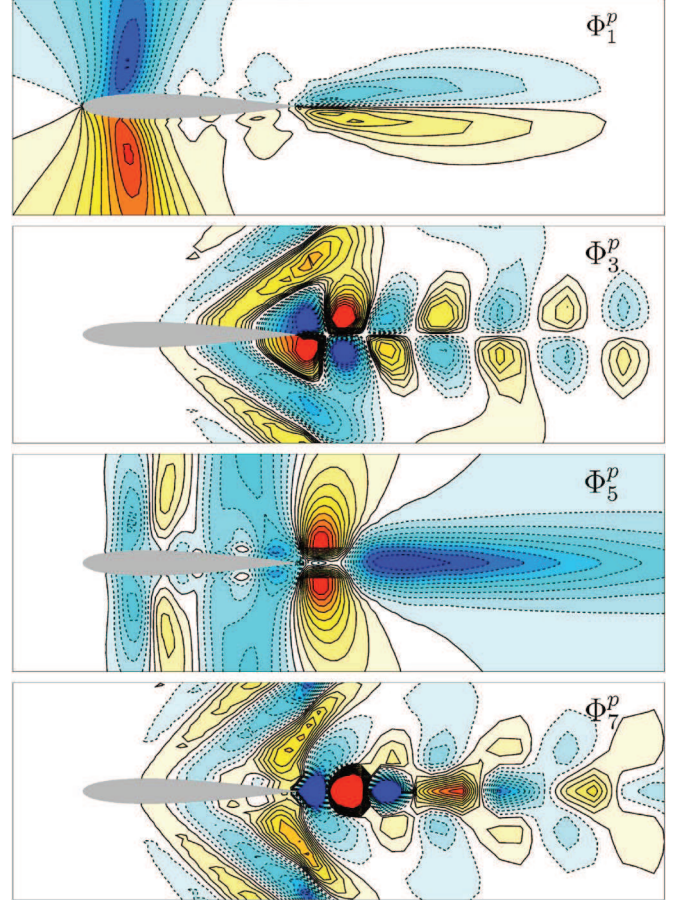
FIG. 3. (Color online) First four odd spatial POD modes associated to pressure in flow A ( \text{Ma}=0.80 , \text{Re}=10^4 ), where the von Kármán instability interacts with the buffet phenomenon. Positive (negative) values are denoted by solid (dashed) lines.
