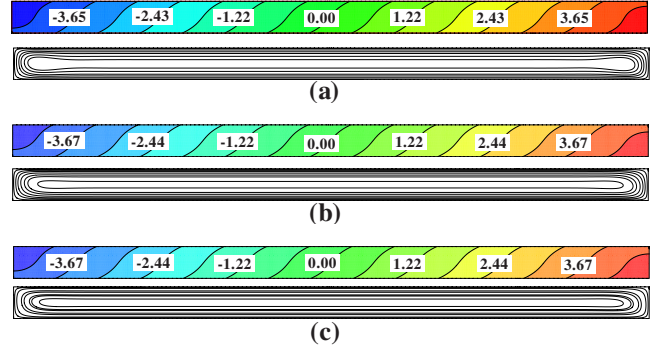
FIG. 5. (Color online) Isoconcentrations and streamlines for the optimal Rayleigh numbers for \psi=0.1 , \varepsilon^*=0.5 and for (a) Le=20 , Ra=12 , (b) Le=100 , Ra=2.4 , and (c) Le=250 , Ra=0.96 .
