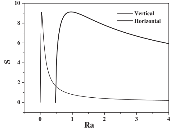
FIG. 8. Separation in horizontal and vertical cells for Le=250 , \psi=0.1 , \varepsilon^*=0.5 .
