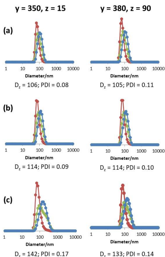
Figure 3. DLS study of core swelling for selected R_0-(SS-Na^+)_{140}-b-Sty-b-DEGDMA_z-SC(S)SnPr CCMs. The measurements were made on filtered solutions ( 0.45 \mu\text{m} pore filter). (a) Unswollen latex. (b) Swollen by toluene. (c) Swollen by chloroform.
