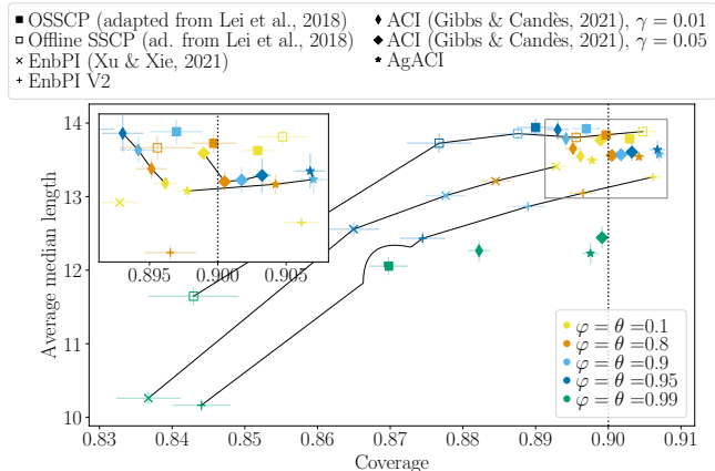
Figure 6. Performance of various CP methods on data simulated according to equation (3) with a Gaussian ARMA(1,1) noise of asymptotic variance 10 (see Appendix C.2). Results aggregated from 500 independent runs. Empirical standard errors displayed.
