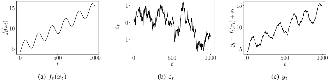
Figure 10. Representation of data simulated according to model A.5.
