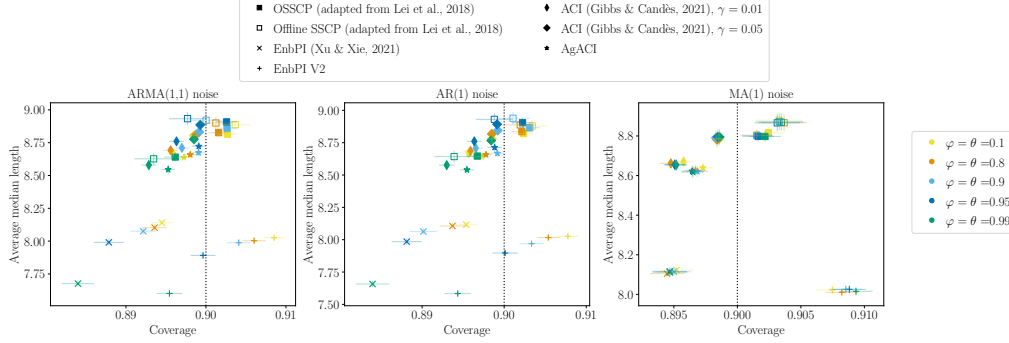
Figure 14: Performance of interval prediction methods on data simulated according to equation (3) with an ARMA(1,1) (left), AR(1) (center) and MA(1) (right) noise with a \mathcal{N}(0, 1 - \frac{\varphi^2}{1 - 2\varphi\theta + \theta^2}) innovation. Results aggregated from 500 independent runs. Empirical standard error are displayed.
