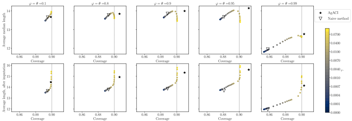
Figure 3: ACI performance with various \theta, \varphi and \gamma on data simulated according to equation (3) with a Gaussian ARMA(1,1) noise of asymptotic variance 10 (see Appendix C.1). Top row: average median length w.r.t. the coverage. Bottom row: average length after imputation w.r.t. the coverage. Stars correspond to the proposed online expert aggregation strategy, AgACI, and empty triangles to the naive choice.
