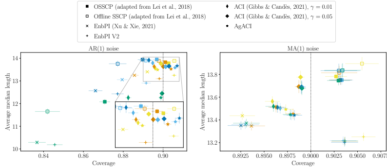
Figure 13: Performance of various interval prediction methods on data simulated according to equation (3) with a Gaussian AR(1) (left) and MA(1) (right) noise of asymptotic variance 10 (see Appendix C.1). Results aggregated from 500 independent runs. Empirical standard error are displayed.
