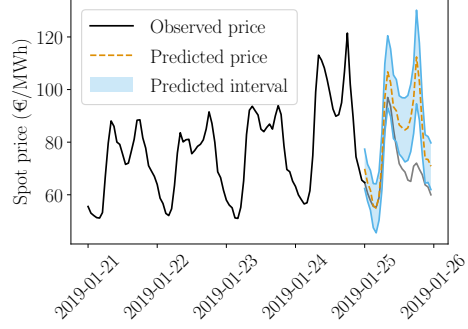
(c) EnbPI V2
