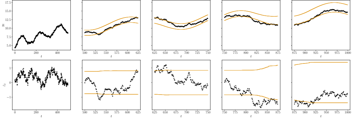
Figure 9: Visualisation of OSSCP on simulated data, from model model A.5. 1000 data points are generated. The 500 first ones form the initial calibration set, displayed on the first subplot of each row. The 500 last ones are the ones the algorithm tries to predict. They are displayed on the 4 last subplots of each row: the second displays response from t = 501 to t = 625 , the third from t = 626 to t = 750 and so on. Observed values are in black, predicted intervals bounds are displayed in orange
