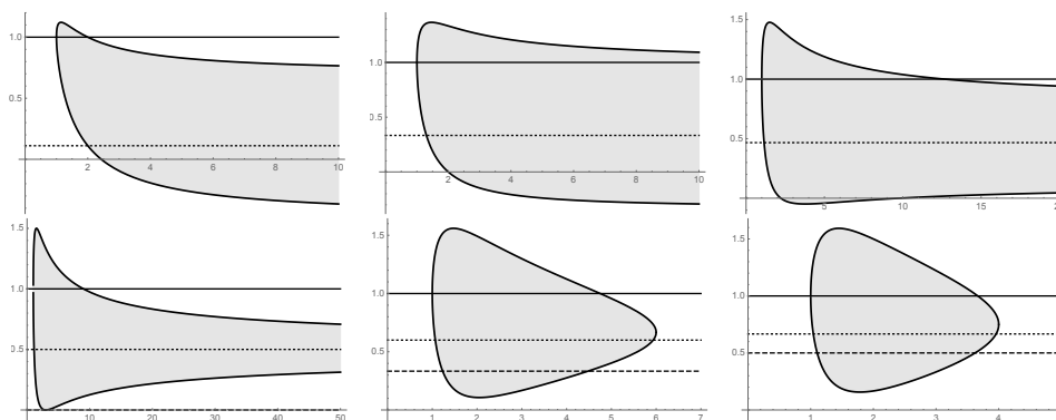
FIGURE 1. Admissible ranges of m for n = 0.25, 1, 1.8 (first line, from the left to the right) and n = 2, 3, 4 (second line). The dotted and dashed curves correspond respectively to m = n/(n+2) and m = (n-2)/n . In Lemma 4, Condition (21) amounts to (n-2)/n < m < 1 and m \neq n/(n+2) .
