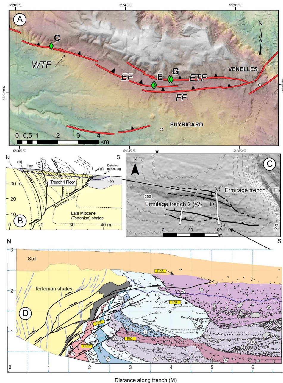
Figure 4. Figures illustrating the Trévèresse paleoseismicity study. (A) Location of faults and of paleoseismicity trenches on the southern limb of the Trévèresse anticline. Trenches names (green diamonds): C = Collavery, E = Ermitage, G = Ganay. Fault Names: WTF: West Trévèresse Fault, ETF: East Trévèresse Fault, EF: Ermitage Fault, FF: La Fauchonne Fault. Location information and fault locations are from Chardon et al. [2005, 2009] and Nguyen et al. [2007]. (B) Middle scale cross section along the Ermitage T1 trench modified from Chardon et al. [2005]. (a), (b), (c) are the location of trenches log presented in Chardon et al. [2005] and also located on the map presented on the Figure 4C. (C) Detailed map on the Ermitage–Ganay area (DEM 1 m resolution, https://geoservices.ign.fr/documentation/diffusion/telechargement-donnees-libres.html#rge-alti-1-m , IGN) showing 1 m spaced level curves. Both trenches T1 and T2 are located. The Ermitage Fault and associated splays are mapped. (D) Southern trench T1 log ((a) on Figures 4B and 4C) modified from Chardon et al. [2005] showing the southernmost fault offsetting the soil of which the base displays a 20 cm reverse offset probably by the 1909 earthquake faulting [Chardon et al. , 2005]. Units (numbered pentagons) 1–7 are interpreted by Chardon et al. [2005, 2009] as colluvial wedges that could be associated with coseismic displacements. Roman numbered triangles identify five fault splays. Chardon et al. [2005] identified an earlier faulting acting on splays I and II and more recent events mobilizing splays III, IV and V. Only splay I and V provide evidence for coseismic surface ruptures. We identified five possible event horizons numbered 1 to 5 on the figure.
