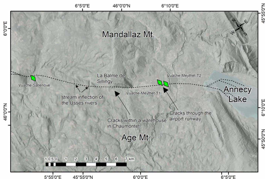
Figure 9. Trench locations indicated with green markers performed in the Anney area. The dotted black line indicates the surface trace of the Vuache fault [De La Taille, 2015]. The stream inflection of the Usses rivers is indicated by arrows [Baize et al. , 2011]. DEM 5 m ( https://geoservices.ign.fr/documentation/diffusion/telechargement-donnees-libres.html#rge-alti-5-m , IGN).
