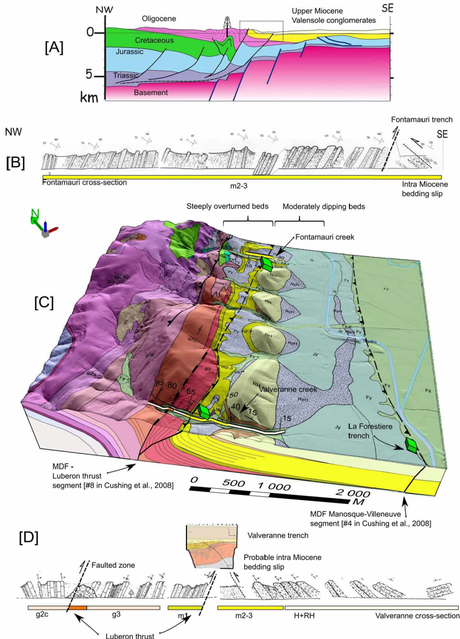
Figure 6. (A) General cross section of the Manosque anticline [adapted from Cushing et al., 2008]. (B) Cross section along the Fontamauri creek showing the overturned beds passing abruptly to conformal geometry at the location of the major fault (Luberon thrust). (C) 3D block showing relationship between the Valvèranne and the Fontamauri trenches/cross sections: both show the same structural setting with a huge reverse fault (Manosque anticline fault) with overturned Oligocene beds at Valvèranne creek and a thick striated gouge zone at Fontamauri. Three green diamonds display locations of trench sites (Valvèranne, La Forestière and Fontamauri). (D) Cross sections along Valvèranne creek shows structure of Oligo-Miocene beds (colored strips for geological stages, g for Oligocene, m for Miocene, H+RH for Miocene Valensole conglomerates). Bedding slip affecting the Miocene series is observed at both sites, in the footwall, of the Fontamauri trench and inferred at the Valvèranne trench. DEM 5 m, https://geoservices.ign.fr/documentation/diffusion/telechargement-donnees-libres.html#rge-alti-5-m , IGN).
