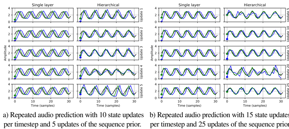
Fig. 3. a) Repeated prediction of a constant sine wave with single layer (left) and hierarchical PCN with two layers (right). The hierarchical model learns a top-down state prior for the sequence, while the single layer model has only local context. When convergence in the lowest layer is not guaranteed, such as with too few gradient descent steps or with inappropriate initialisation of precision, only the hierarchical model correctly tracks the incoming signal. b) With increased gradient steps for state inference in the lowest layer both single-layer and hierarchical PCN eventually show accurate posterior predictions (green). Predictions from the state prior (blue) improve only for the hierarchical model.
