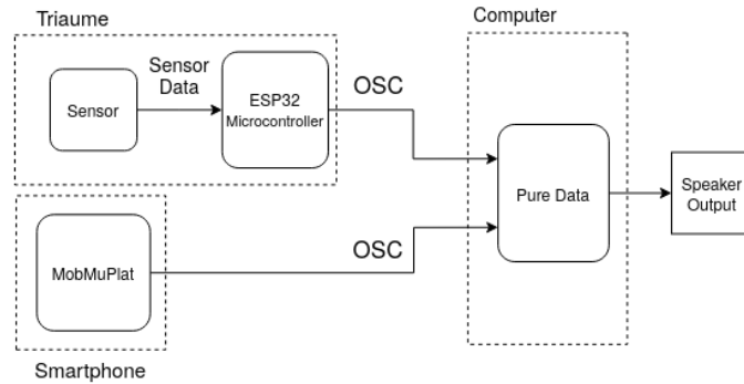
Fig. 1. System overview. The computer receives OSC packets both from the Triahme and from a smartphone.
