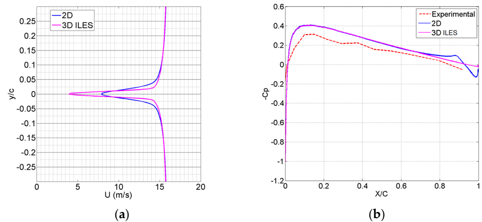
Figure 3. (a) Near-wake U-velocity profile and (b) comparison of predicted vs. measured surface pressure coefficient. Baseline case for NACA-0012 at a 0^\circ AoA and U = 16 m/s.
