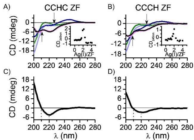
Figure 4. CD titrations of 25 μM metal-free A) CCHC ZF (examined in this study) and B) CCCH ZF (data obtained previously) [27] in 20 mM TES buffer (pH 7.0) with AgNO 3 solution. The light blue, green, dark blue, magenta, and black lines indicate 0, 1, 2, 3, and 4 equivalents of added Ag I , respectively. Arrows indicate observable isodichroic points. The insets represent the CD signal at 245 nm as a function of the Ag I -to-ZF molar ratio. C) and D) the differential spectra obtained by subtraction of metal-free CCHC and CCCH ZF CD spectrum from fully Ag I -loaded CCHC and CCCH ZF spectrum, respectively. The dotted lines represent ellipticity changes at 210 and 220 nm.
