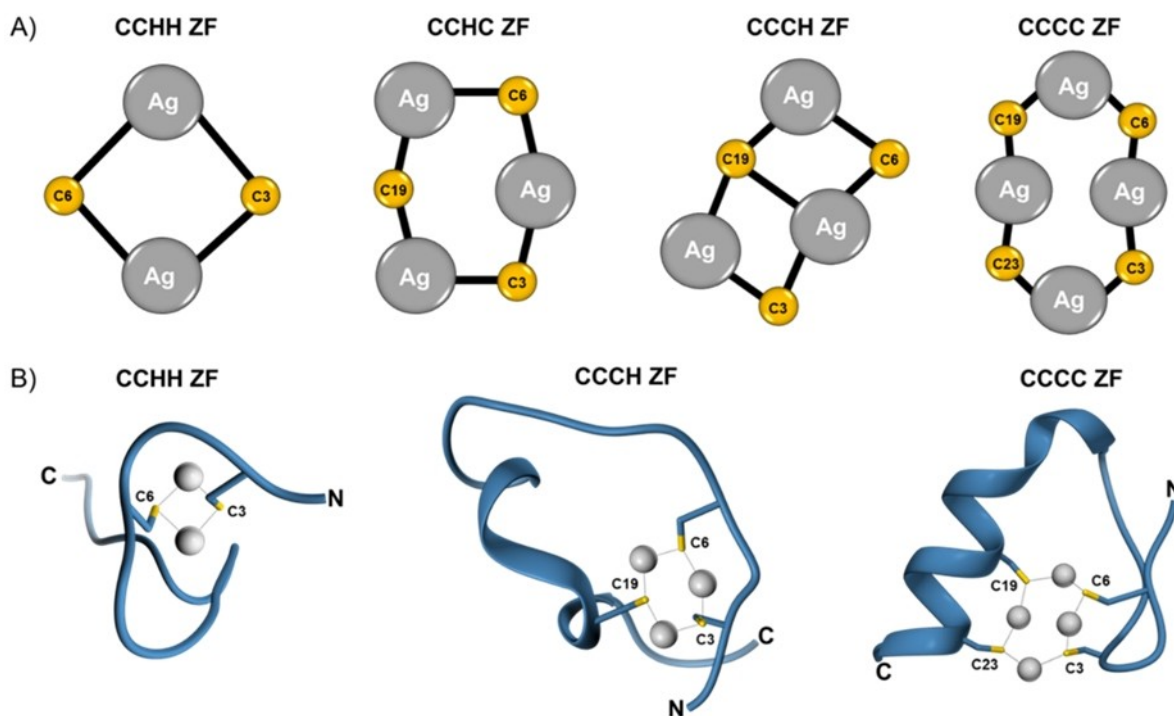
Figure 3. Structural features of Ag I -ZFs. A) Proposed structure of Ag n S n ZF clusters probed in this study by EXAFS analysis. Each cysteine residue is numbered in accordance with ZF sequences from Figure 1B. B) Model structures of Ag n S n ZF clusters obtained by QM/MM MD-based simulations. [27] C and N denote the C- and N-terminal end of ZFs, respectively.
