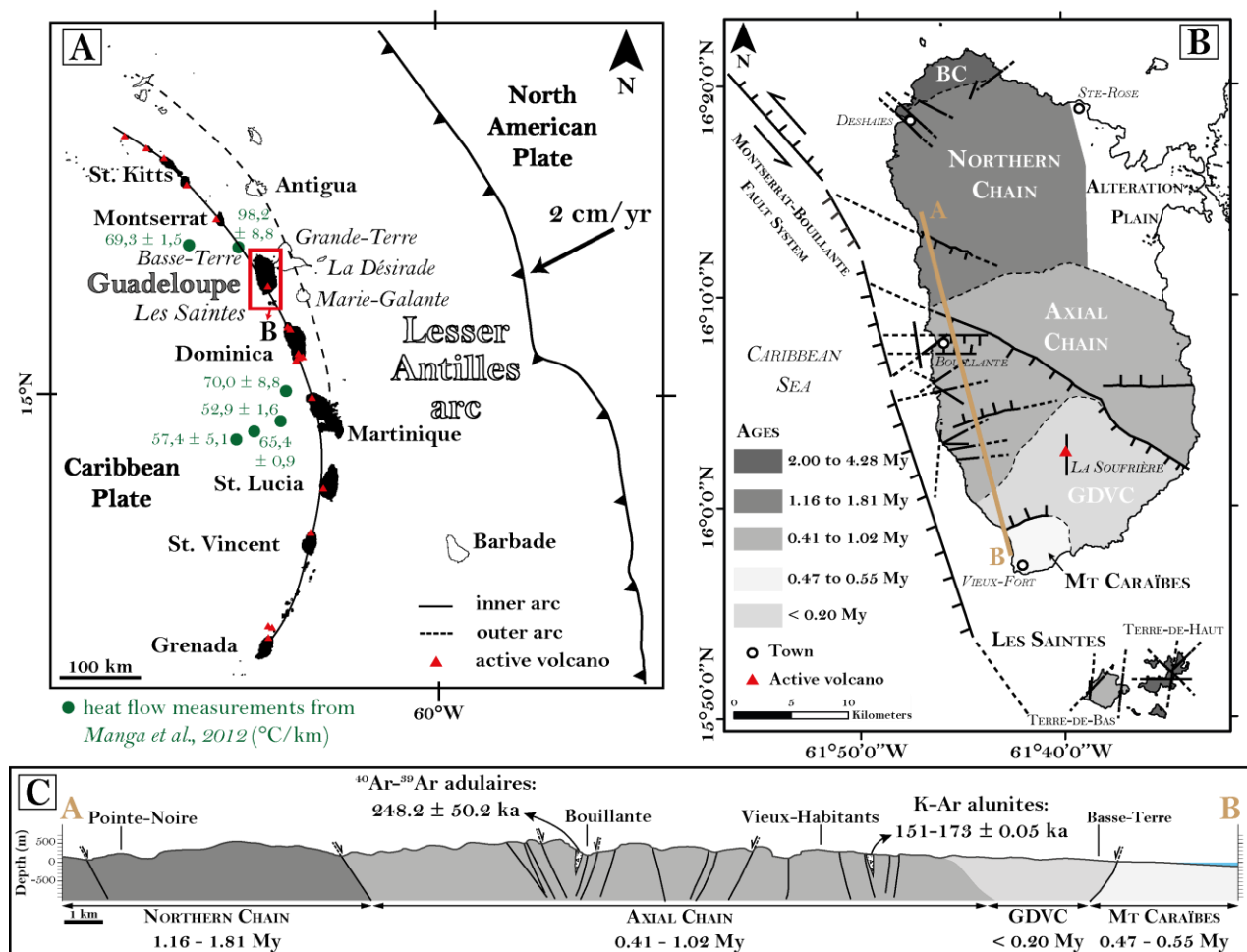
Figure 1: A) Geodynamic setting of the Lesser Antilles arc (after Feuillet et al., 2001), B) Map of the active volcanic arc in Guadeloupe archipelago (i.e. Basse-Terre and Les Saintes) displaying the different volcanic complexes and the main tectonic structures modified after Verati et al. (2018) (BC= Basal Complex, GDVC= Grande Decouverte Volcanic Complex), C) Cross-section NNW-SSE from Basse-Terre island (location in fig 1-B) displaying the spatio-temporal distribution of brittle structures, volcanic complexes and hydrothermal breccias (Ar-Ar dating from Verati et al., 2014 and K-Ar from this study).
