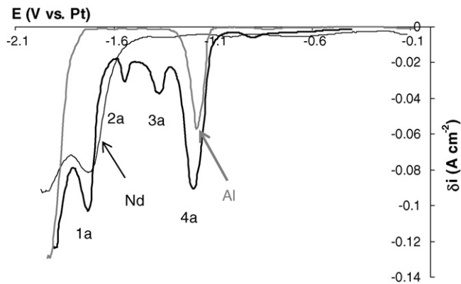
Fig. 8. Square wave voltammogram of the LiF-CaF_2-AlF_3-NdF_3 system compared to LiF-CaF_2-AlF_3 and LiF-CaF_2-NdF_3 systems on Ta electrode at T = 800^\circ C and 0.1 V/s ; auxiliary electrode: vitreous carbon; potential reference: Pt.
