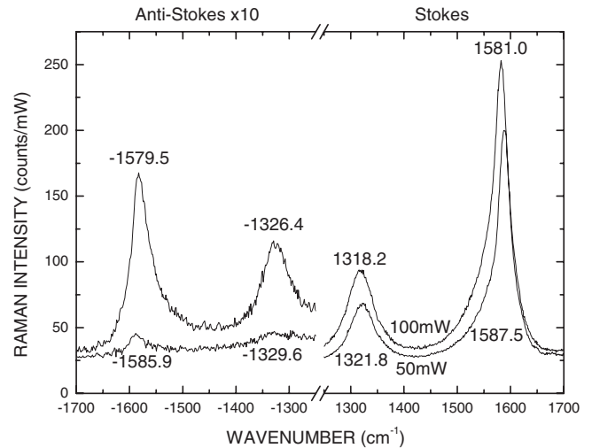
FIG. 4. Raman spectra of DWs recorded with 50 and 100 mW (633 nm). The spectra are scaled to the incident laser power. The anti-Stokes spectra have been multiplied by a factor of 10.
