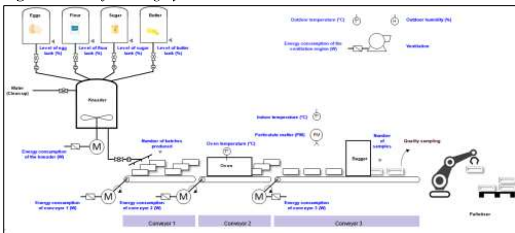
Figure 2. Manufacturing System
