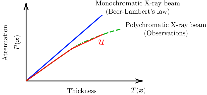
Figure 1: Differences between monochromatic assumptions (blue line), and polychromatic measurements (green dashed line). The aim is to determine the relationship between the two curves through the fit of a parametric function u (red line) to observed data.
