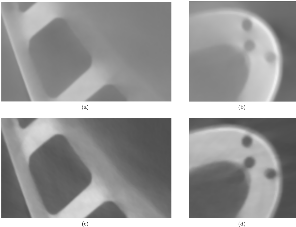
Figure 10: Tomographic volumes using (a) and (b) uncorrected projections, (c) and (d) projections corrected with the identified function u^{-1} .
