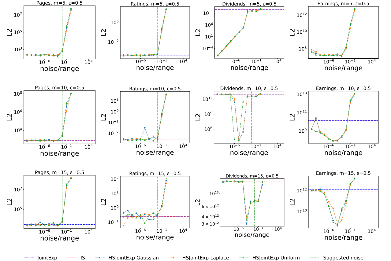
n = 1000 , \epsilon = 0.5 , \mathbf{p} = \left(\frac{1}{m+1}, \dots, \frac{m}{m+1}\right) , L2 = \text{MSE} between the private estimator and the quantiles of the dataset averaged over 100 runs. noise/range indicates the ratio between the standard deviation of the noise and the range of the data. Vertical bars indicate the level of noise that we recommend. Horizontal bars indicate the L2 scores that achieved respectively JointExp and the Inverse Sensitivity mechanism (indistinguishable on some plots).
