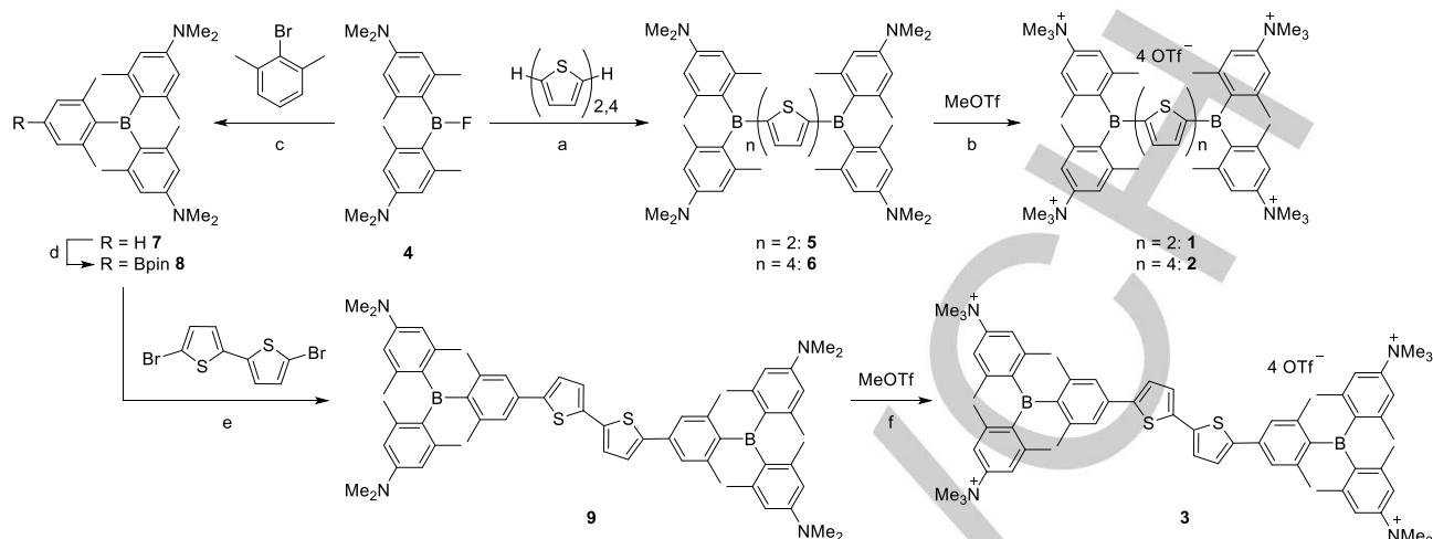
Scheme 1. Synthesis of the compounds 1-3 . a) n -BuLi, THF, -78^{\circ}\text{C} to r.t.; b) \text{CH}_2\text{Cl}_2 , r.t.; c) t -BuLi, THF, -78^{\circ}\text{C} to r.t.; d) \text{B}_2\text{pin}_2 , [\text{Ir}(\mu\text{-OMe})(\text{COD})_2] , dtbpy, THF, 80^{\circ}\text{C} ; e) \text{Pd}_2(\text{dba})_3 , SPhos, KOH, toluene, \text{H}_2\text{O} , 85^{\circ}\text{C} ; f) MeOTf, \text{CH}_2\text{Cl}_2/\text{Et}_2\text{O} 1:3, r.t.
