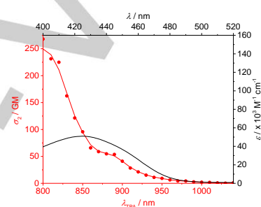
Figure 3. One-photon absorption (OPA) (black) and two-photon absorption (TPA) spectra (red) of 3 in H 2 O.
