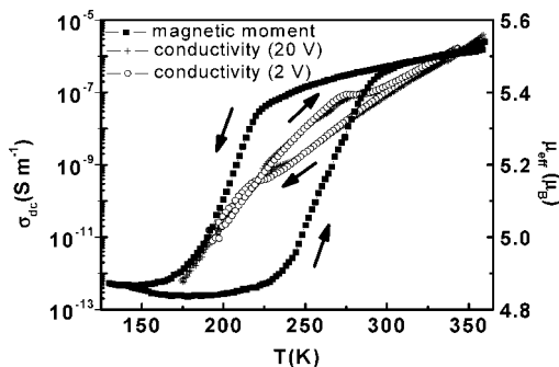
Figure 2. Temperature dependences of the dc conductivity (measured at 2 and 20 V bias) and the effective magnetic moment for sample 1.
